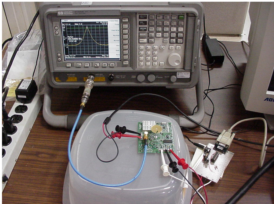
Figure 6 – Setup for Direct Output Power measurements
