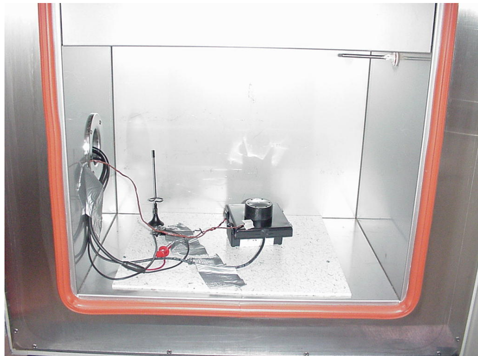
Figure 4 – Internal view of Temperature Chamber Setup
