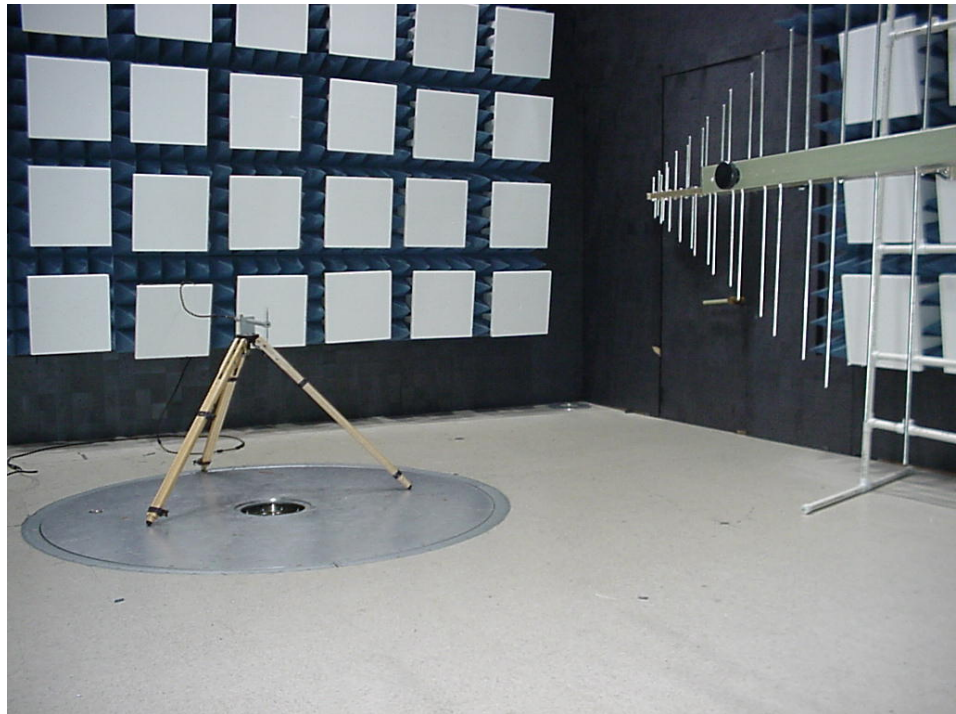
Figure 5 – Setup for Substitution Method
