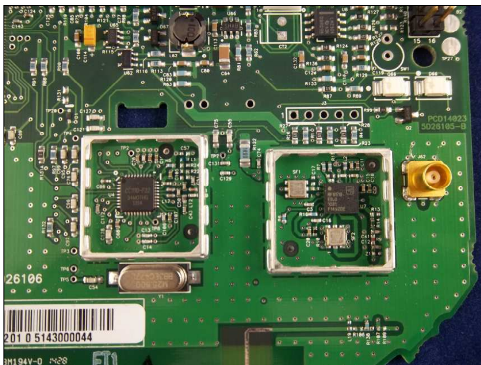
Figure 6: Internal Photo – Shields Removed
