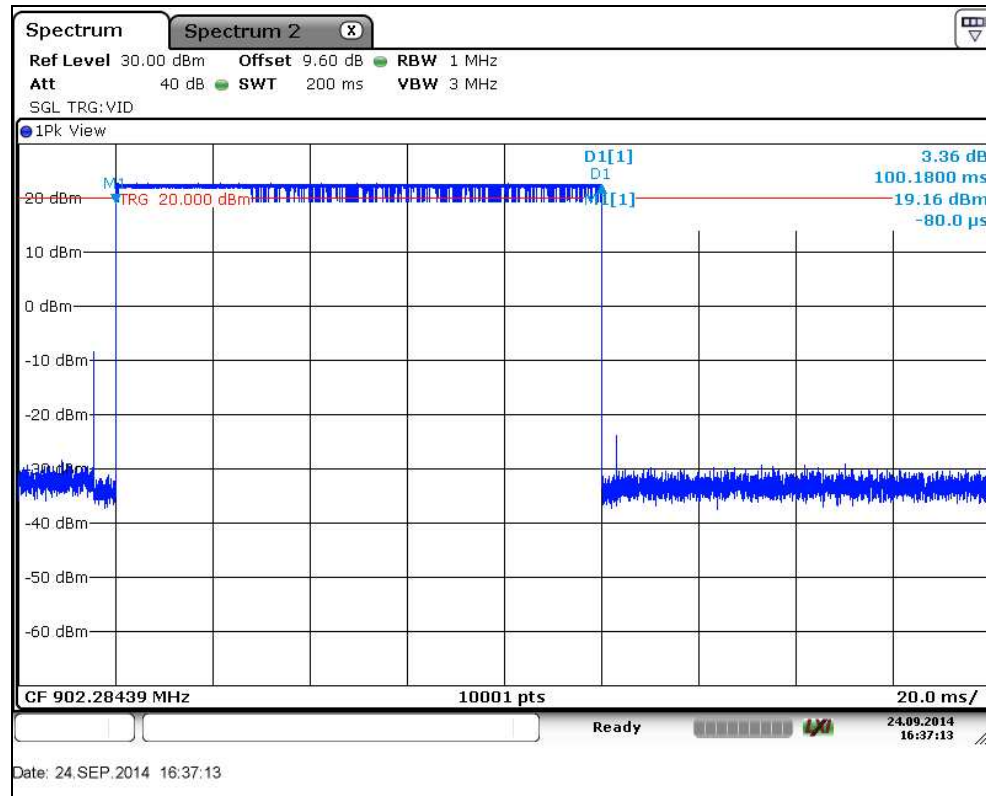
Figure 7.4.3.2-1: Dwell Time
