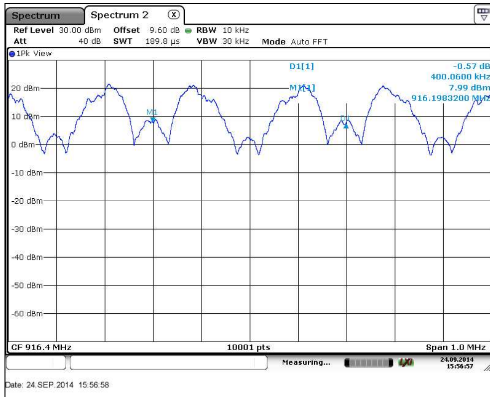
Figure 7.4.1.2-1: Carrier Frequency
