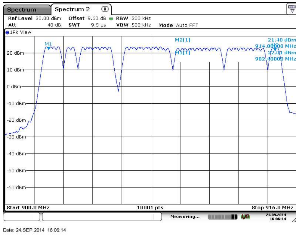
Figure 7.4.2.2-1: Number of Hopping Channels (Lower Band)
