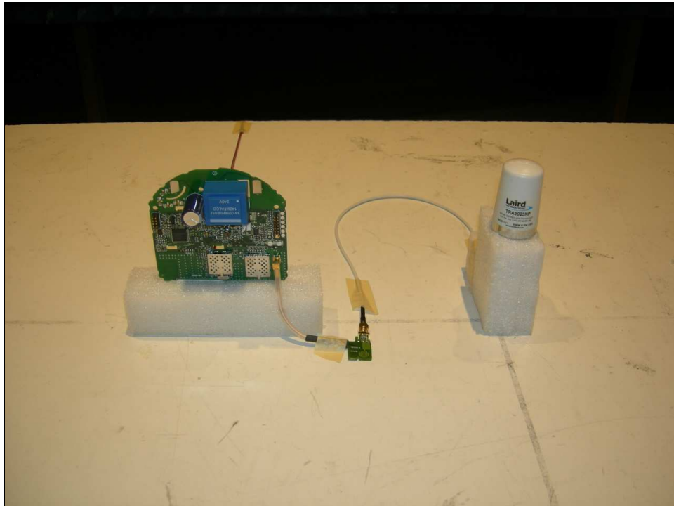
Figure 3: Radiated Emissions – Stubby Antenna
