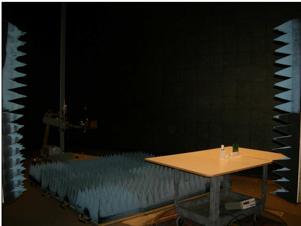
Figure 4: Radiated Emissions – Stubby Antenna
