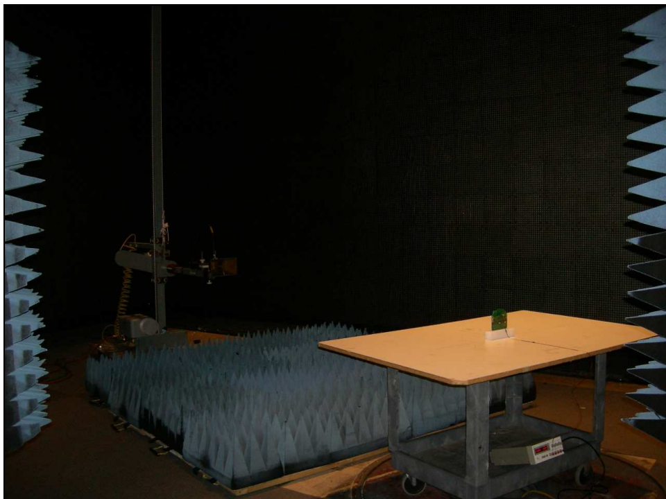
Figure 6: Radiated Emissions – Internal Antenna
