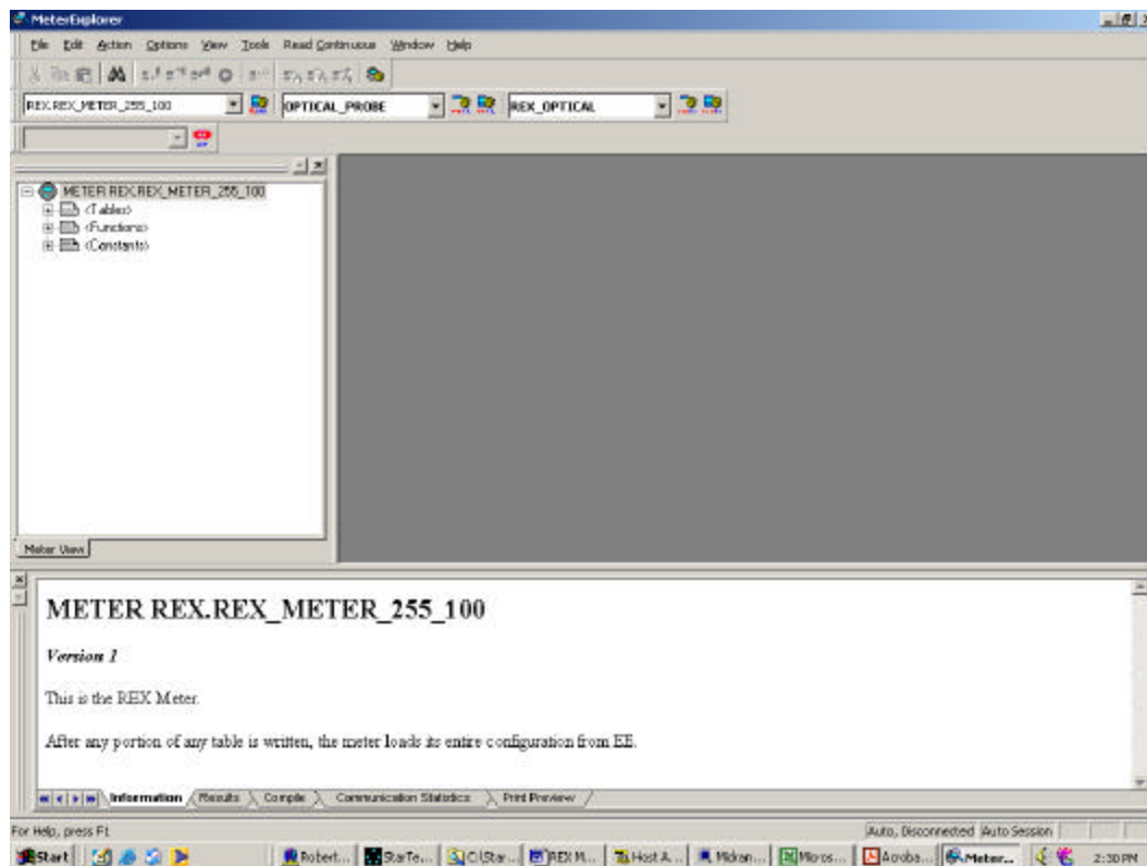
Figure 17: MeterExplorer GUI
