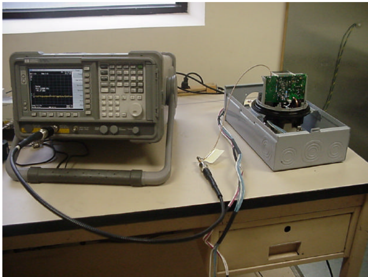
Figure 10 – Setup for Conducted Power Measurements
