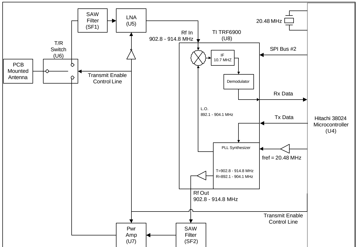
Figure 14: Radio Block Diagram
