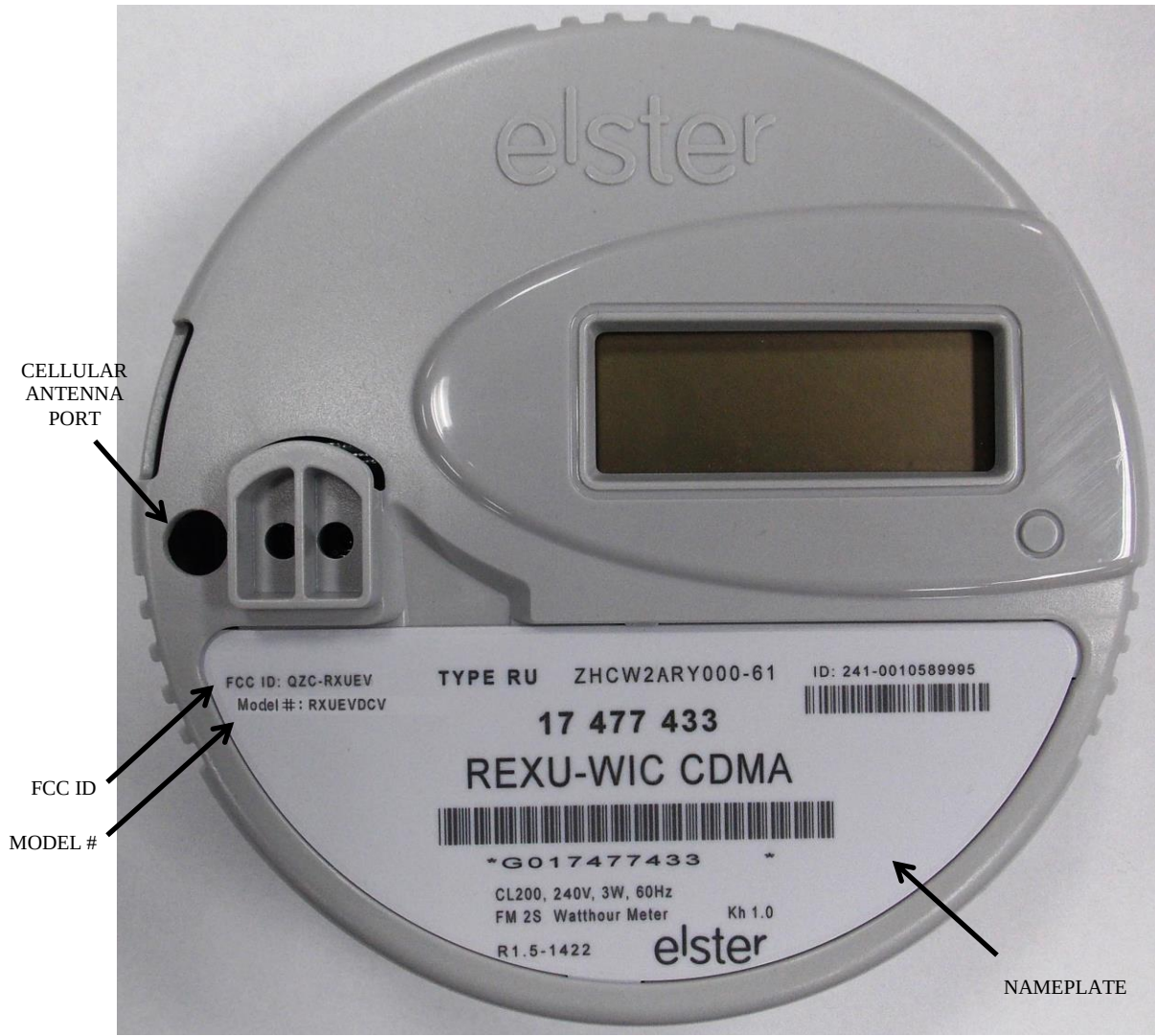
REXUniversal® WWIC cellular antenna port and nameplate info
