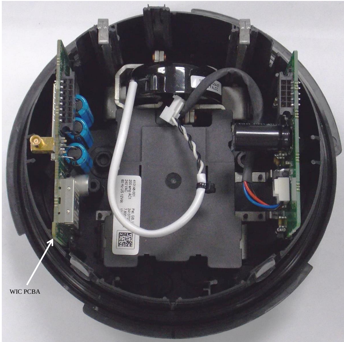
REXUniversal® Form 2S meter base w/disconnect & WIC PCBA (Model # RXUEVDCV)
