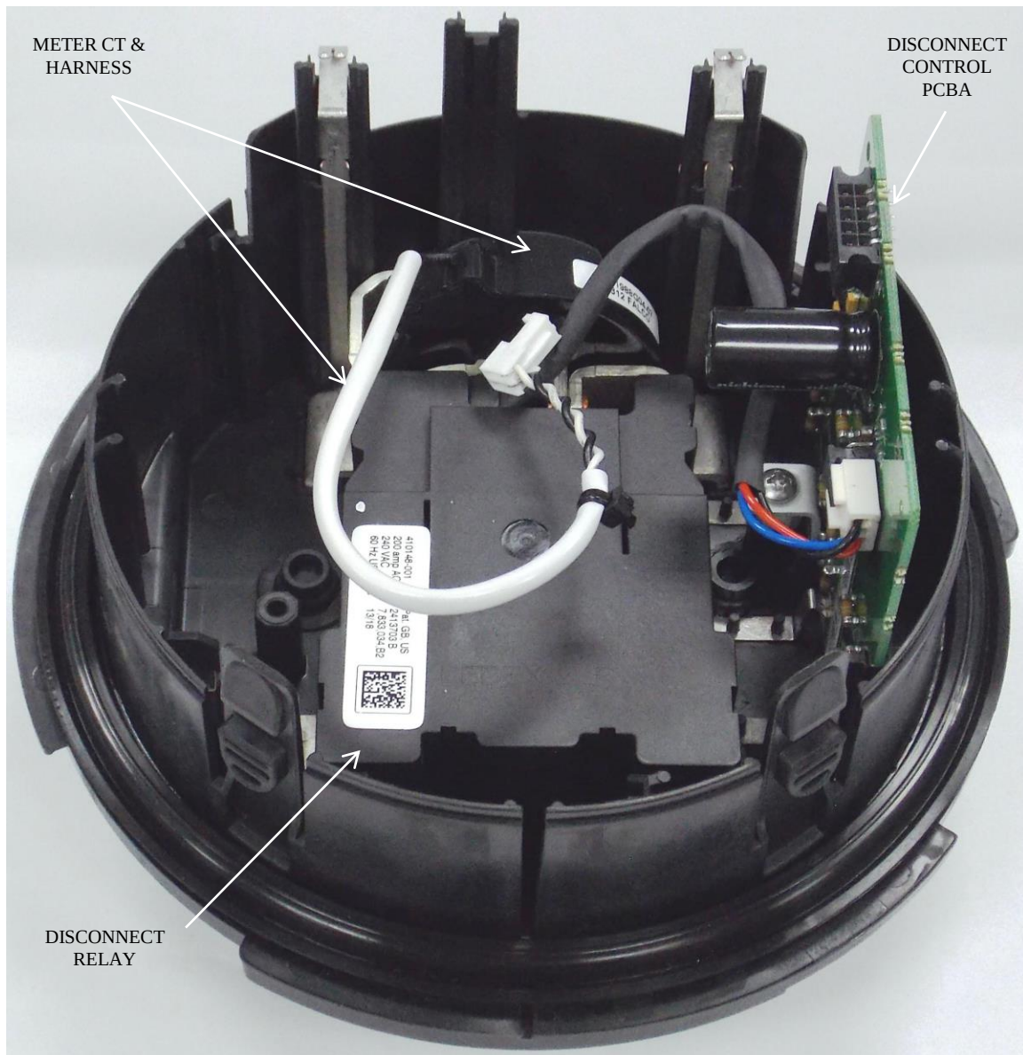
REXUniversal® Form 2S meter base w/disconnect (Model # RXUEVDCV)
