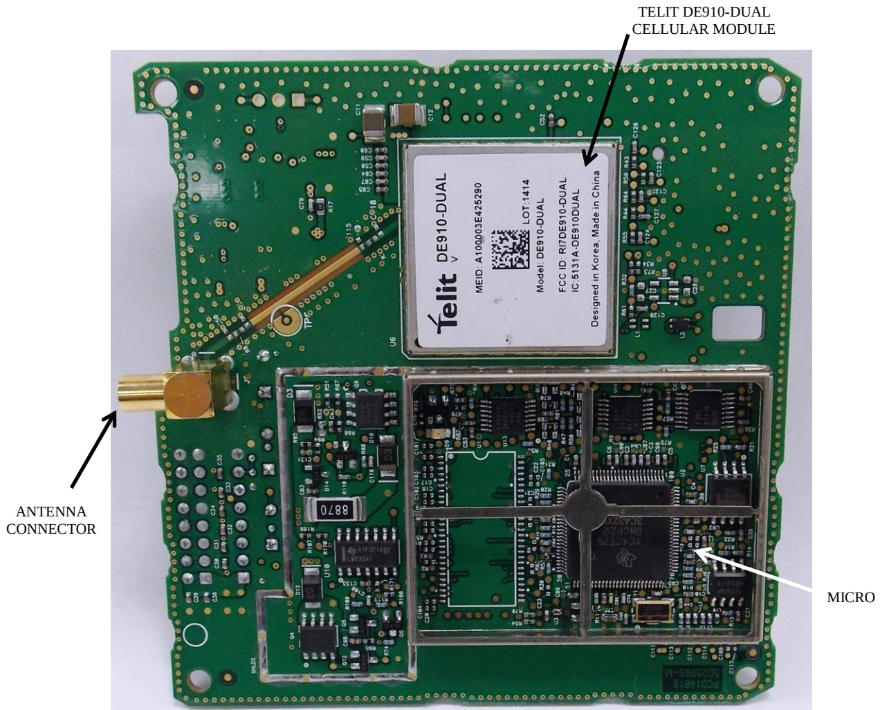
REXU WWIC3G PCBA bottom side view
