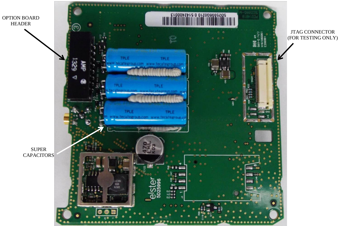
REXU WWIC3G PCBA top side view
