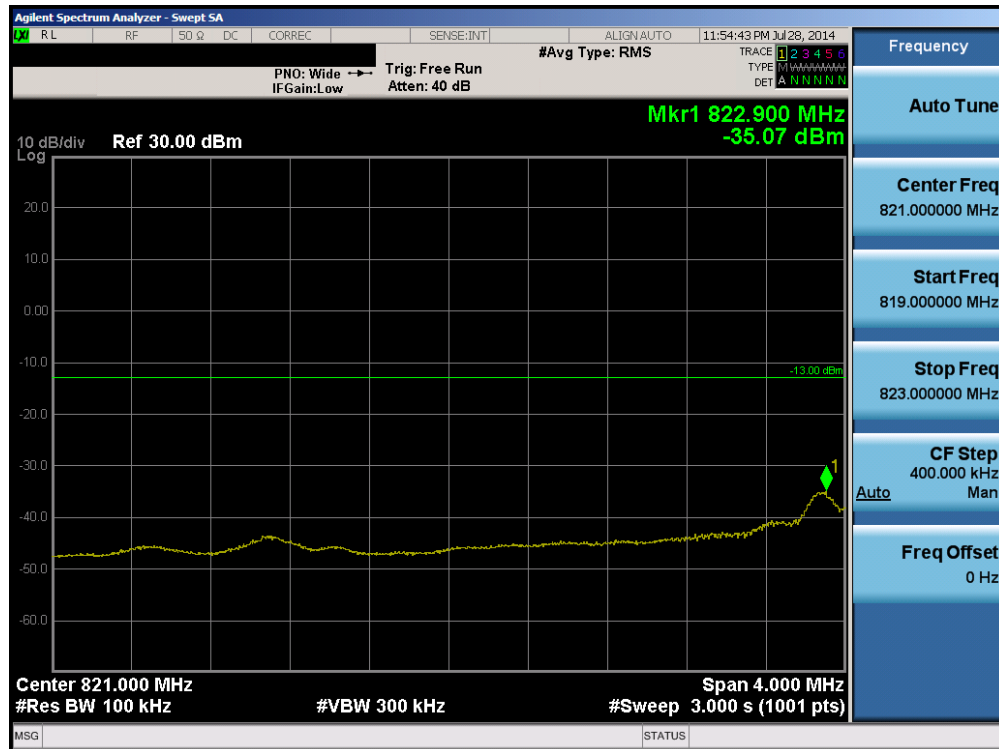
Plot 6-16. 4MHz Span Plot (Cellular CDMA Mode – Ch. 1013)
