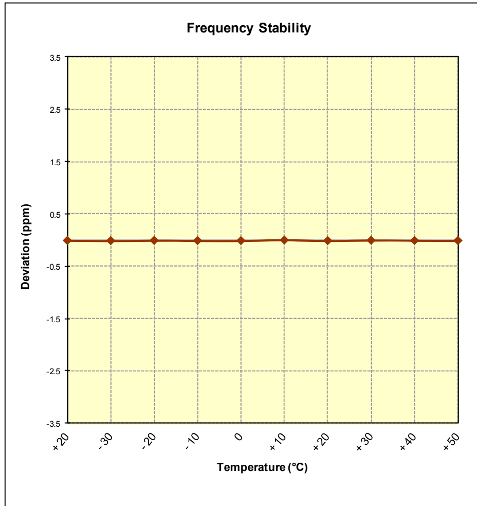
Figure 6-9. Frequency Stability Graph (PCS CDMA Mode – Ch. 600)
