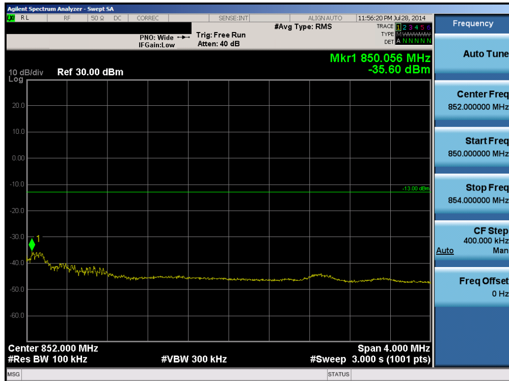
Plot 6-18. 4MHz Span Plot (Cellular CDMA Mode – Ch. 777)
