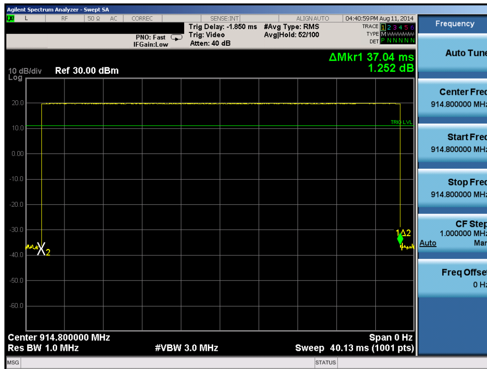
Plot 6-12. Time of Occupancy Plot (900MHz Band)
