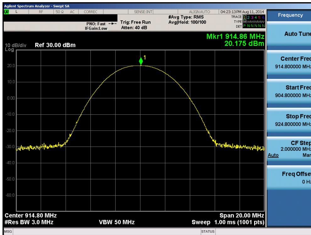
Plot 6-5. Peak Conducted Power (Ch. 31)
