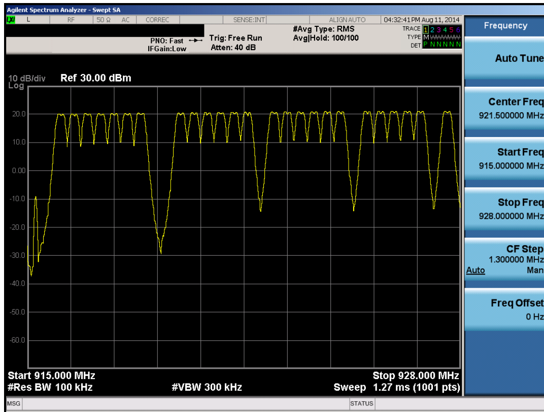
Plot 6-15. High End Spectrum Channel Hopping Plot
