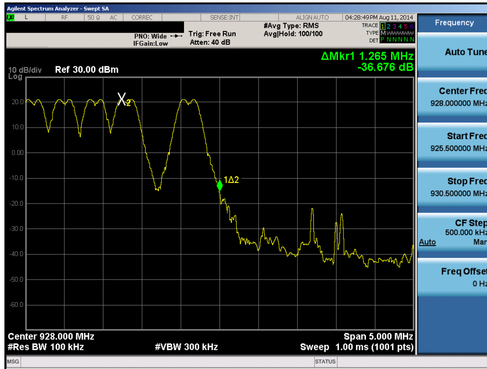
Plot 6-10. Band Edge Plot (Hopping Enabled)
