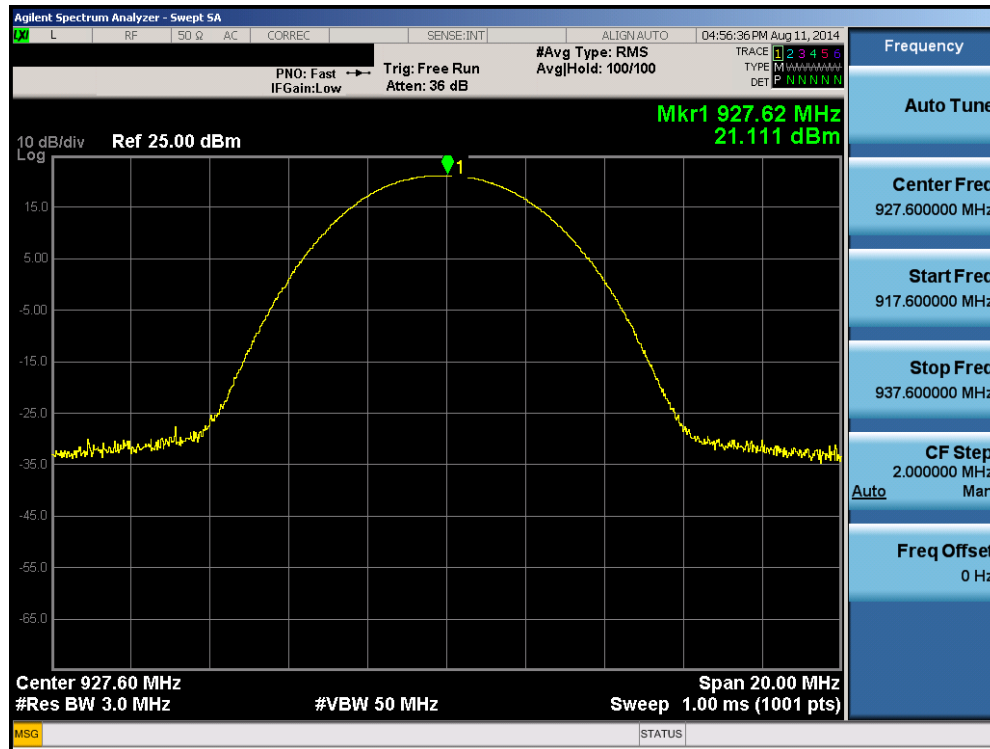
Plot 6-6. Peak Conducted Power (Ch. 63)
