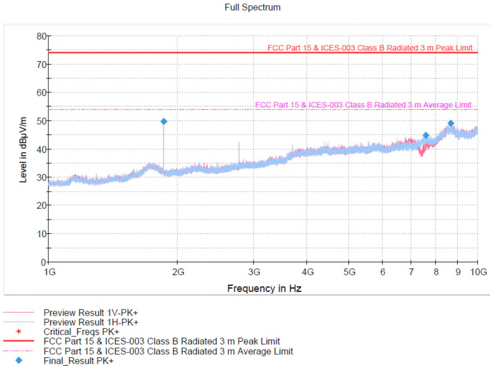
Figure 7.5.3.3-4: Radiated Spurious Emissions Prescan – Mode 2 – Above 1GHz
