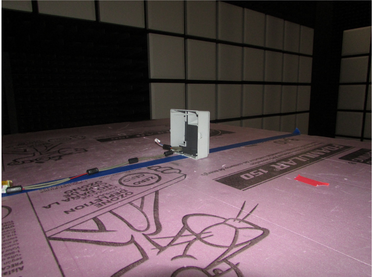
Figure 5: Radiated Emissions – Front – Above 1GHz - XPOS
