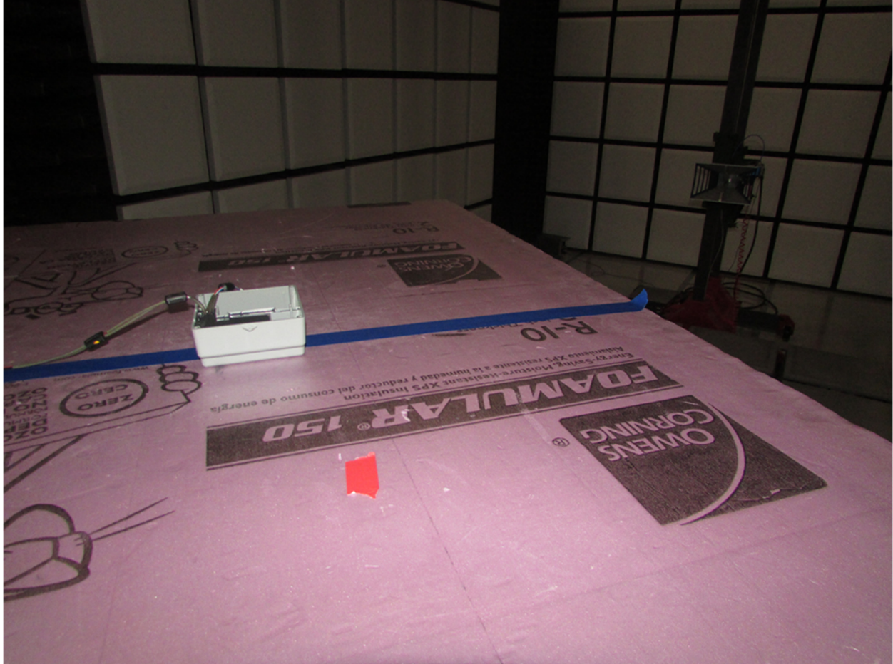
Figure 4: Radiated Emissions – Back – Above 1GHz – ZPOS
