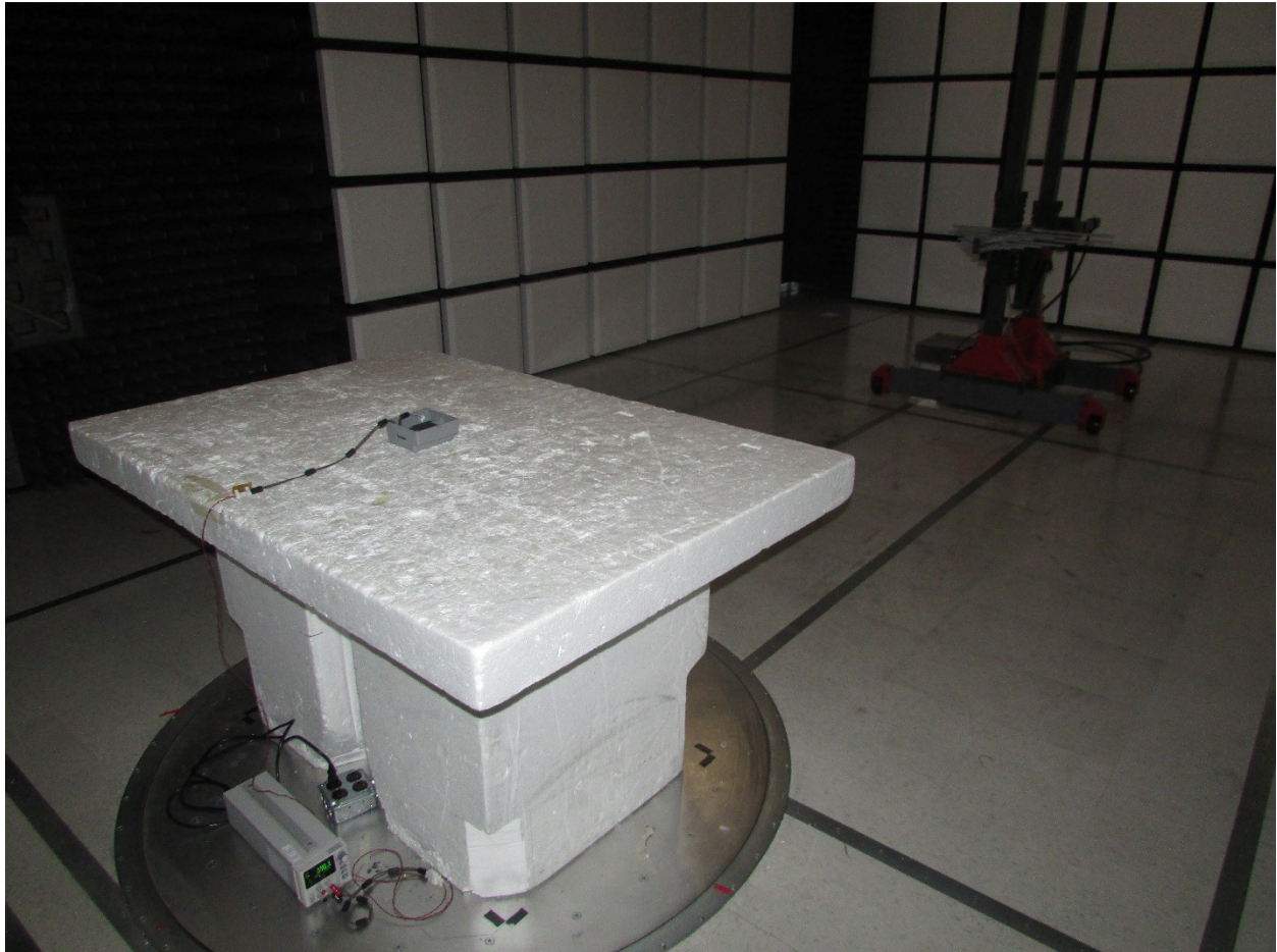
Figure 1: Radiated Emissions – Front – Below 1GHz
