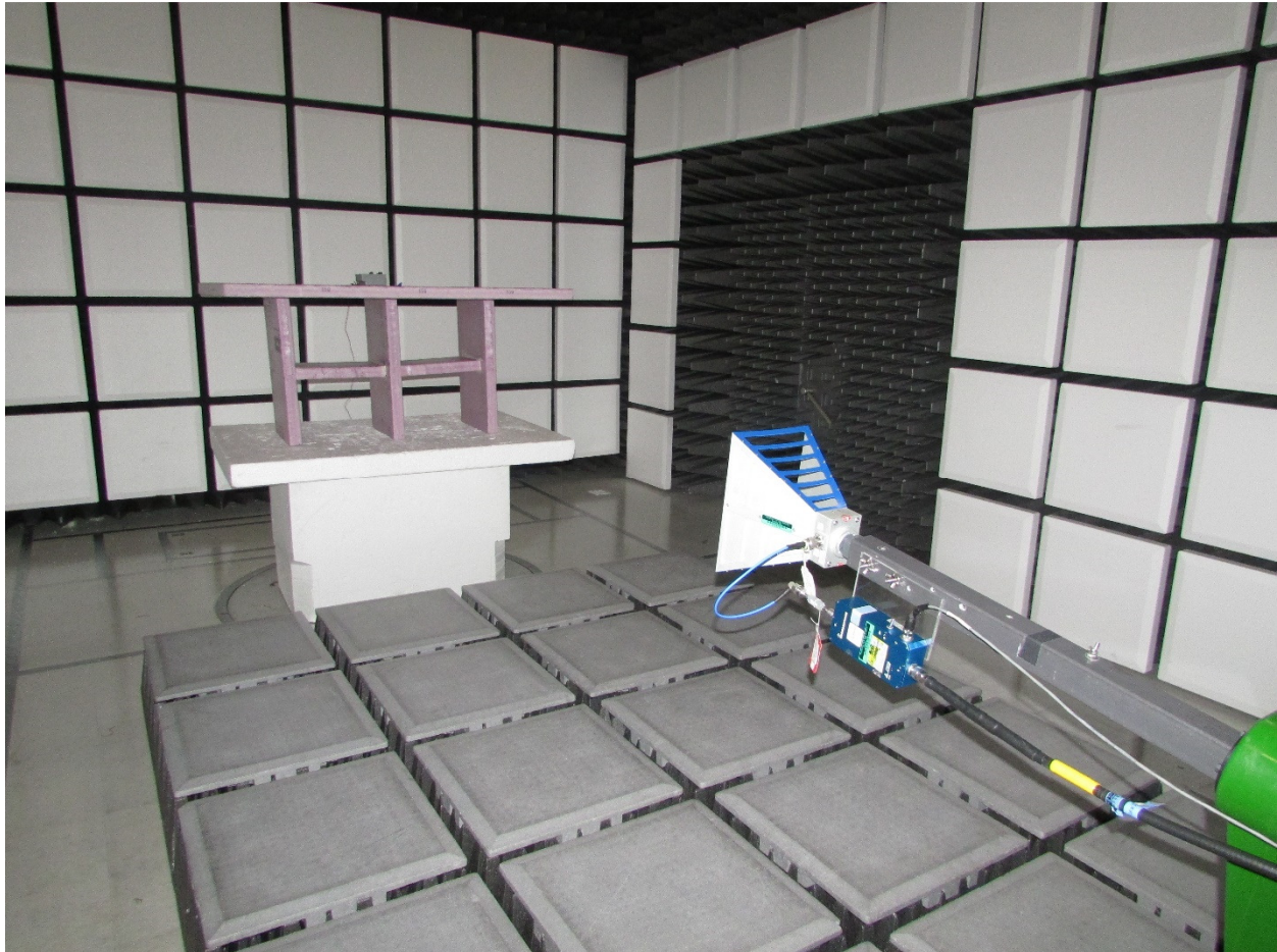
Figure 3: Radiated Emissions – Front – Above 1GHz- ZPOS
