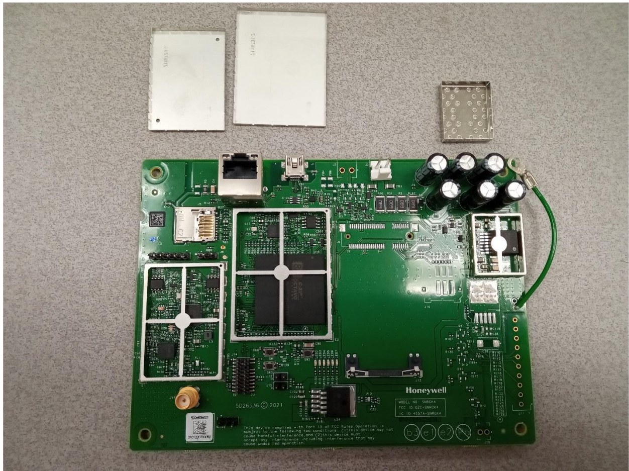
SNRGK4 PCBA Top Side, shield cans off
