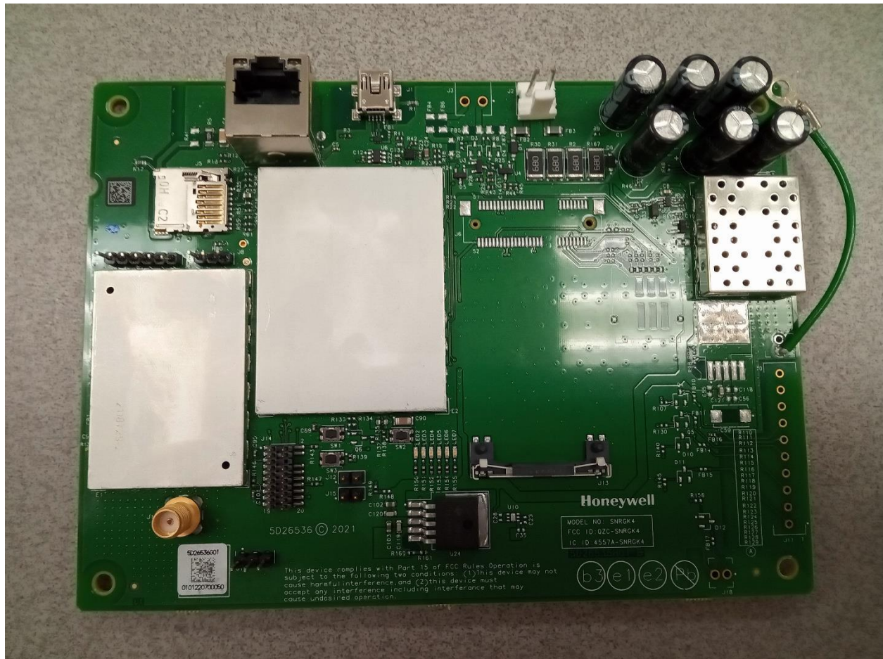
SNRGK4 PCBA Top Side, shield cans on
