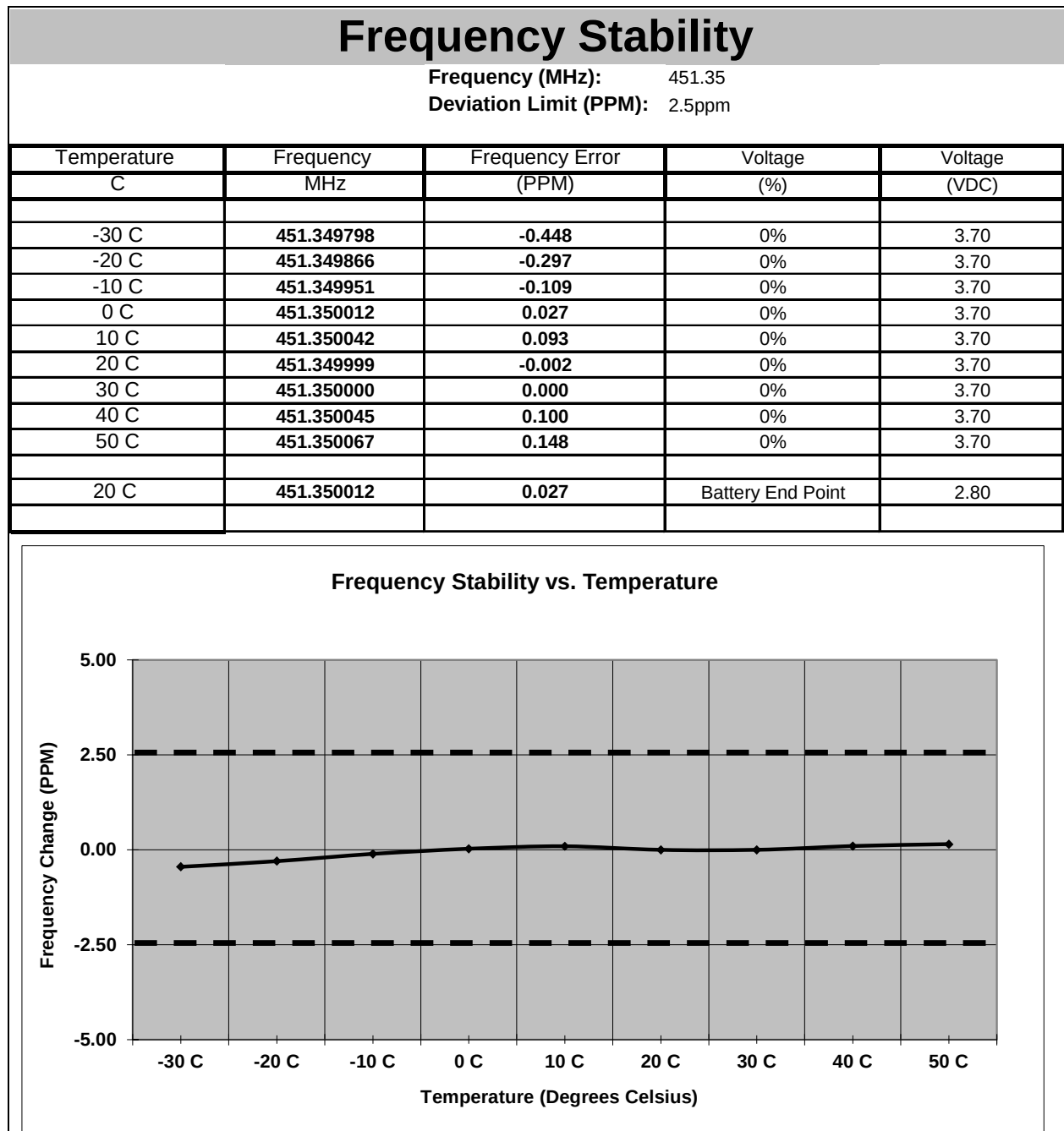
Figure 7.6.2-1: Frequency Stability
