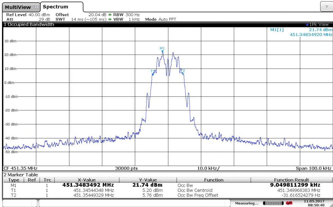
Figure 7.3.2-1: 451.35MHz – 2GFSK
