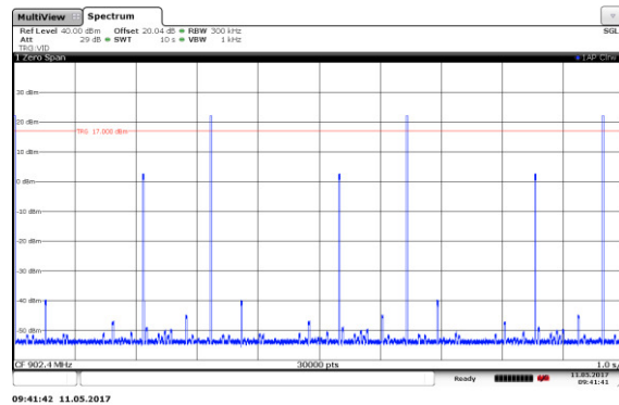
Figure 7.4.3.2-2: Number of Hops – 200kbps
