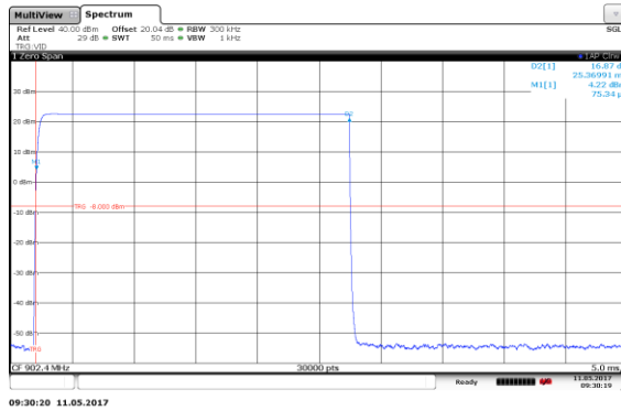
Figure 7.4.3.2-1: Dwell Time – 50kbps
