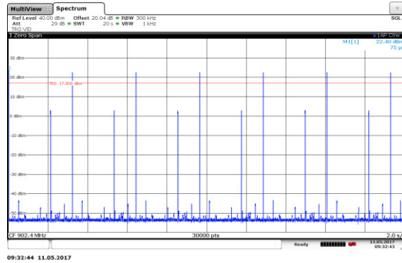
Figure 7.4.3.2-2: Number of Hops – 50kbps
