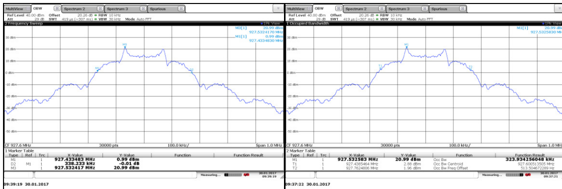
Figure 7.4.4.2-25: 20dB BW High Channel – 142.2 kbps
