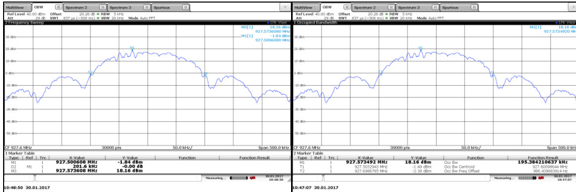
Figure 7.4.4.2-27: 20dB BW High Channel – 150 kbps
