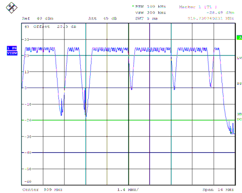
Figure 7.4.2.2-1: Number of Hopping Channels – 35.35 kbps
