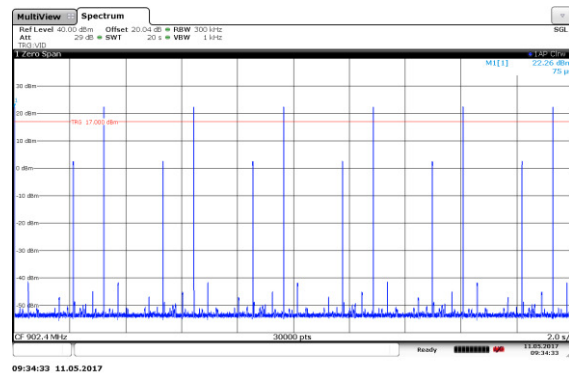
Figure 7.4.3.2-2: Number of Hops – 150kbps
