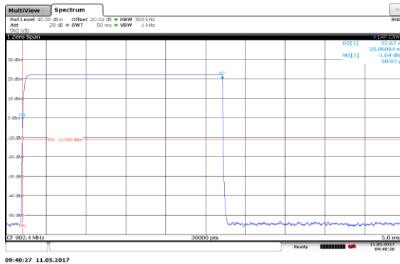
Figure 7.4.3.2-1: Dwell Time – 200kbps
