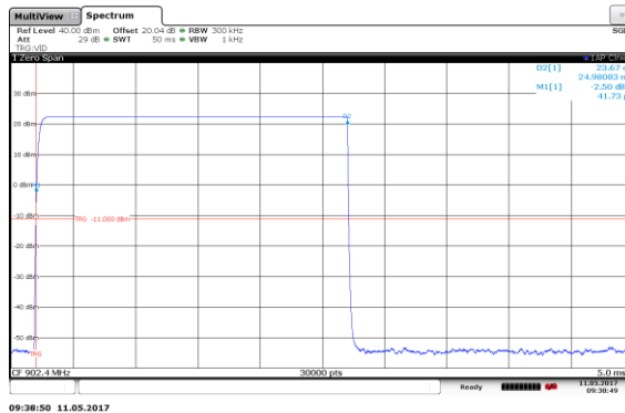
Figure 7.4.3.2-1: Dwell Time – 150kbps
