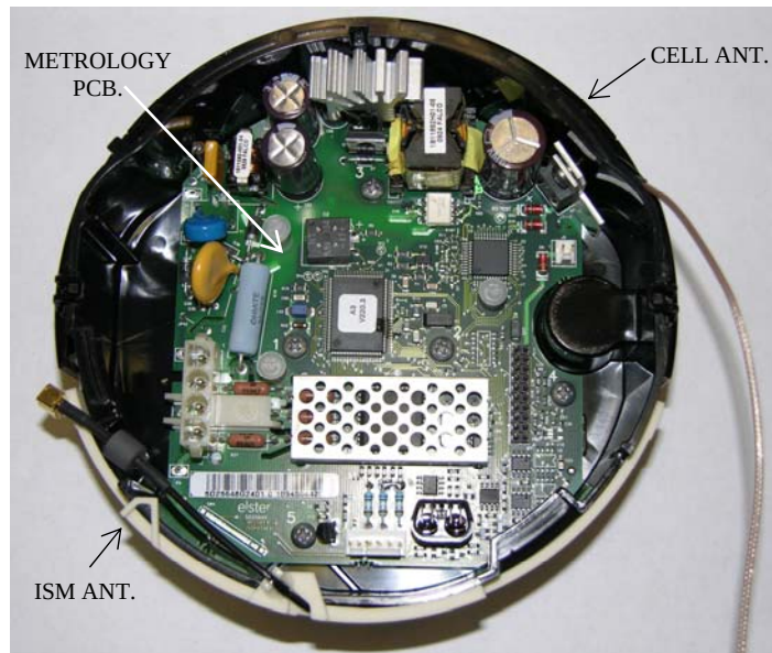
EA_Gatekeeper base module with LAN/WAN antennas
