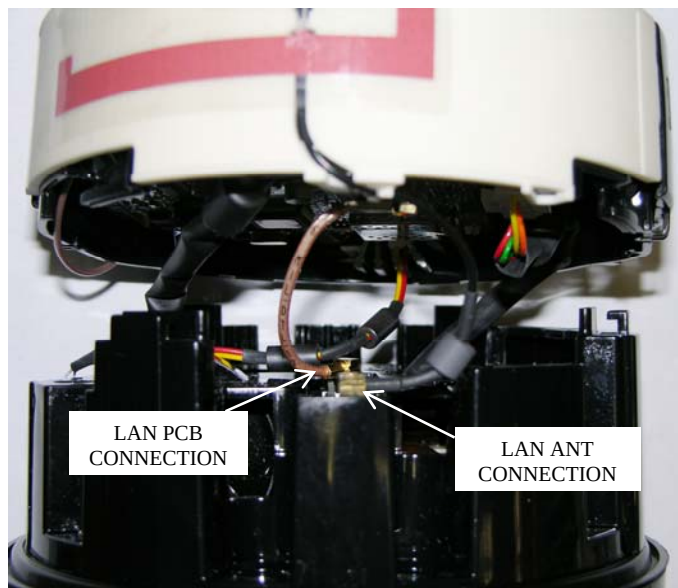
EA_Gatekeeper complete module with RF filter connections
