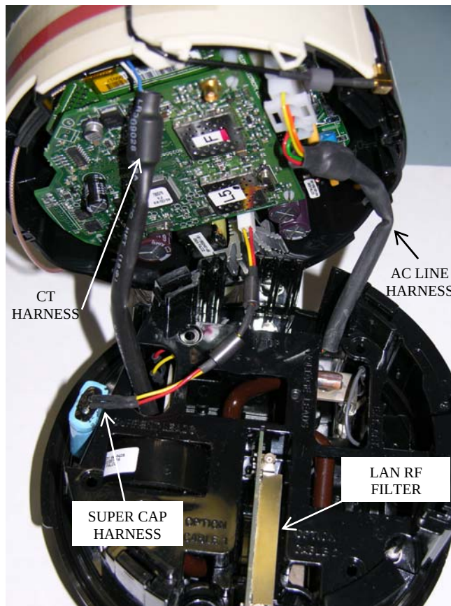
EA_Gatekeeper complete module with meter base
