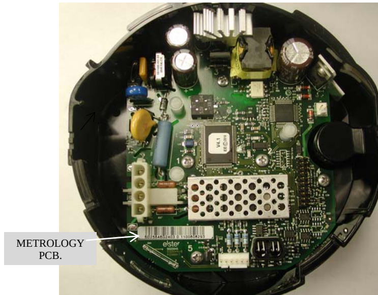
EA_Gatekeeper base module
