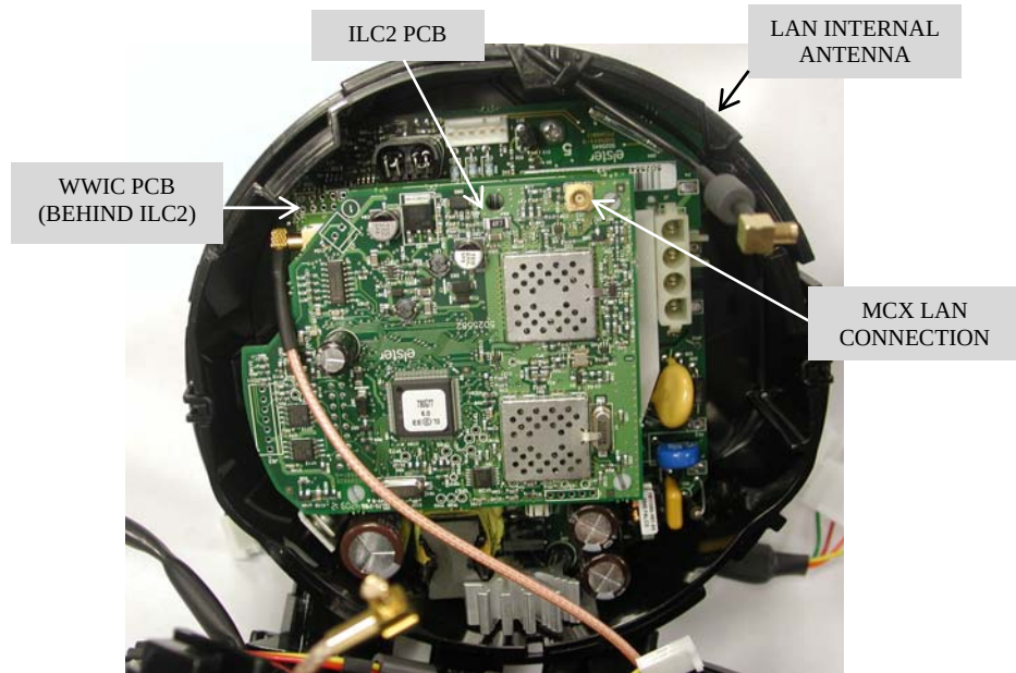
EA_Gatekeeper base module with WWIC and ILC2 PCB installed
