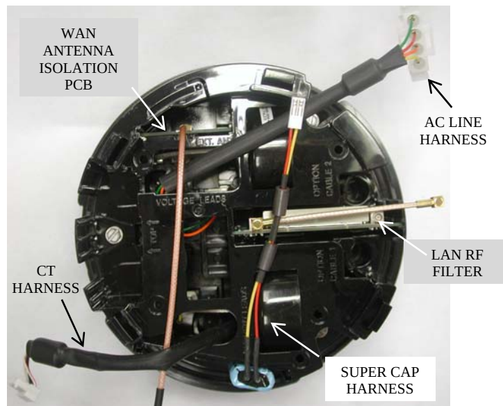
EA_Gatekeeper meter base assembly
