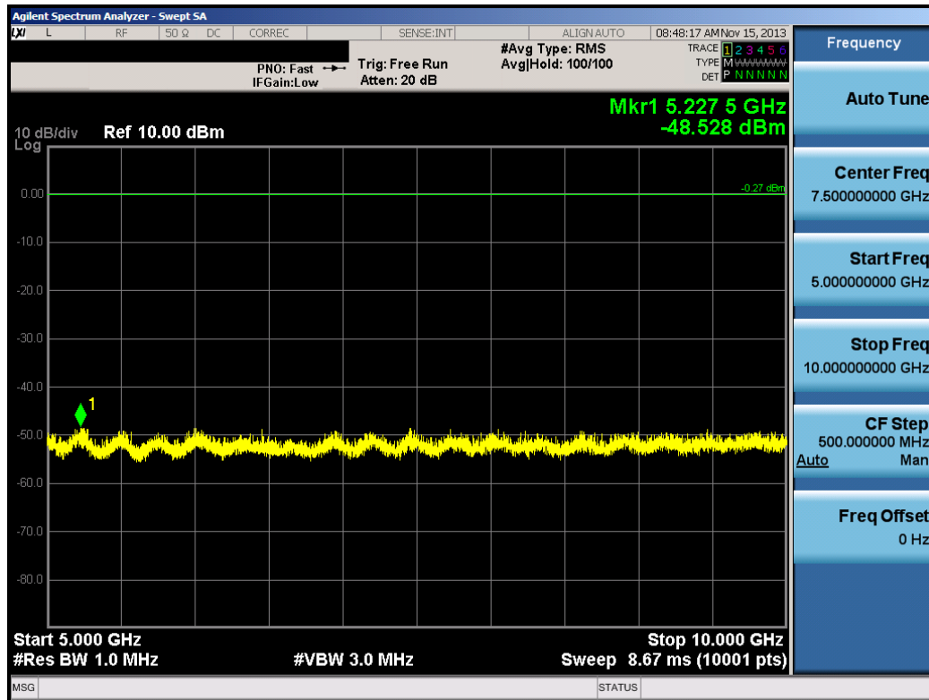
Plot 6-17. Conducted Spurious Plot (900MHz ISM Band – Ch. 1)
