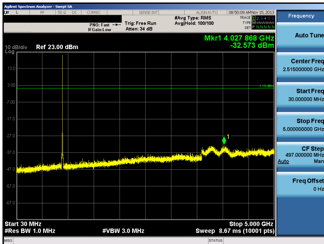
Plot 6-18. Conducted Spurious Plot (900MHz ISM Band – Ch. 31)
