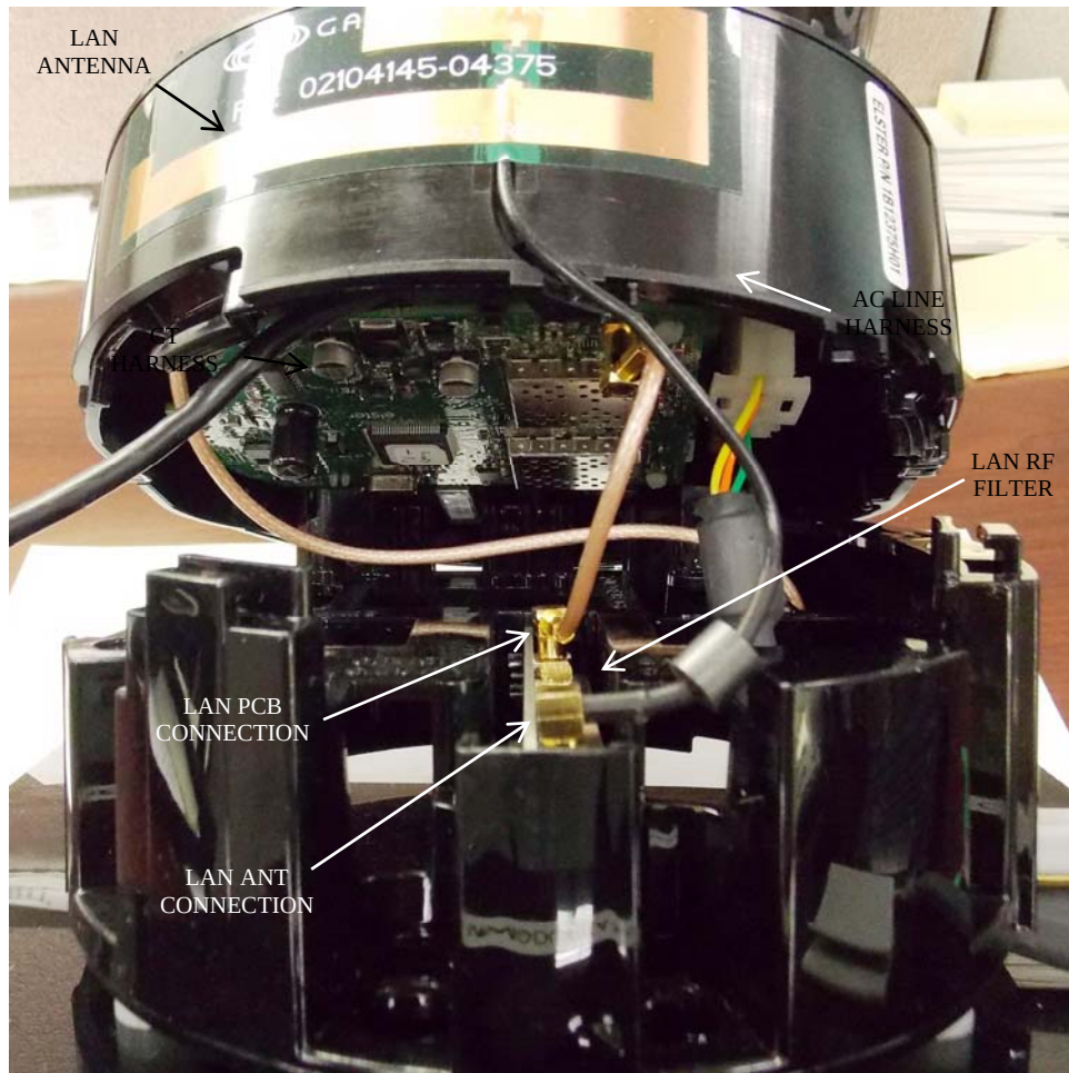
Modular EA_Gatekeeper complete module with meter base
