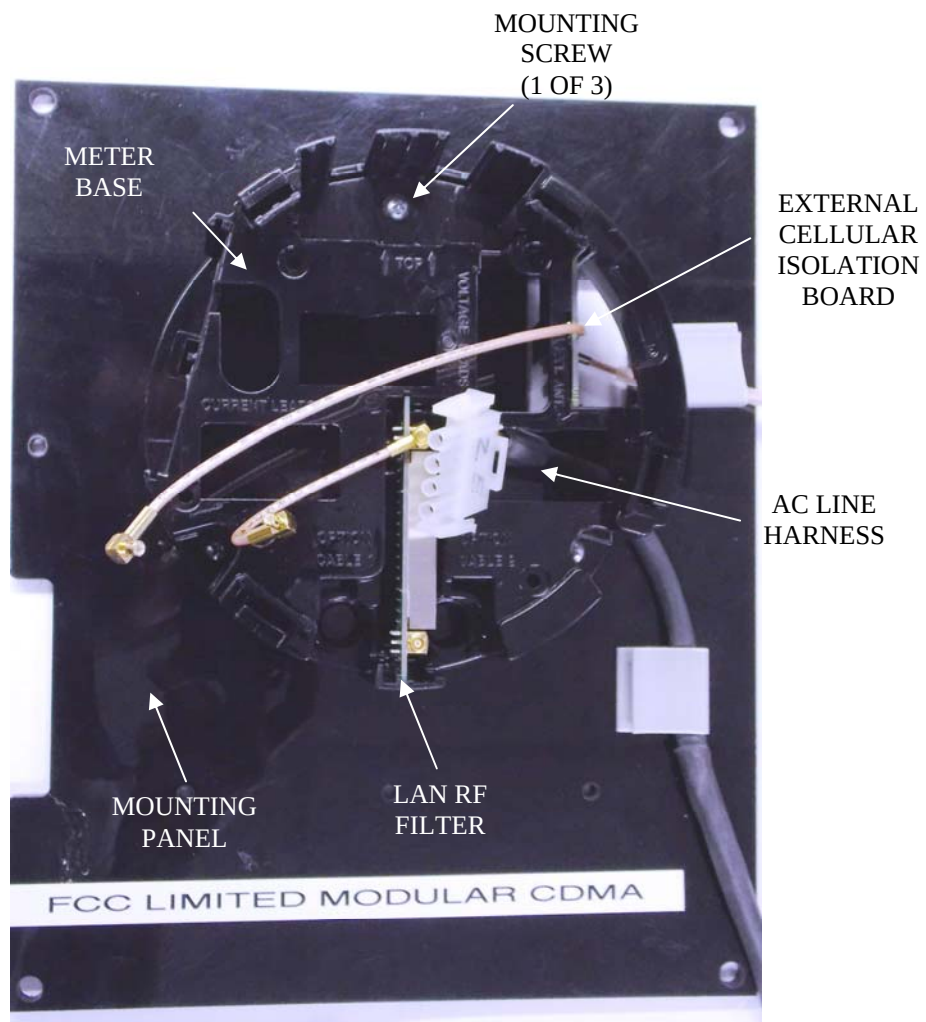
Modular EA_Gatekeeper base on plastic panel
