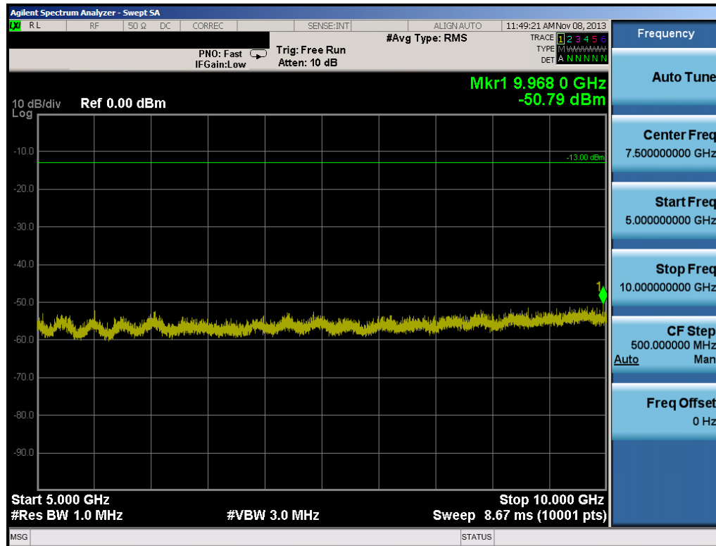
Plot 6-4. Conducted Spurious Plot (Cellular CDMA Mode – Ch. 1013)
