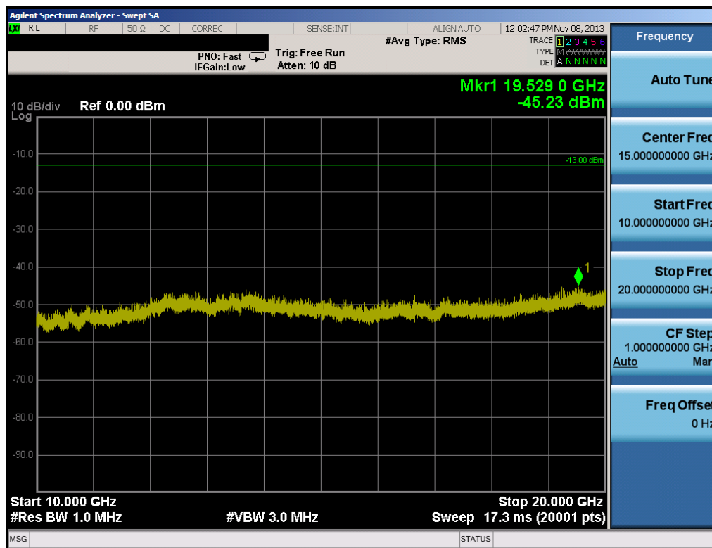
Plot 6-14. Conducted Spurious Plot (PCS CDMA Mode – Ch. 1175)
