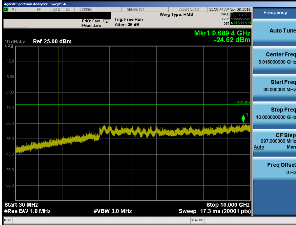
Plot 6-9. Conducted Spurious Plot (PCS CDMA Mode – Ch. 25)
