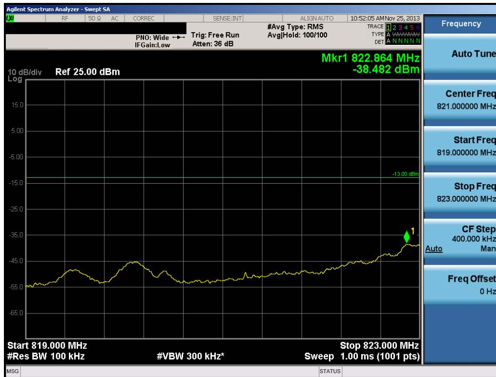
Plot 6-16. 4MHz Span Plot (Cellular CDMA Mode – Ch. 1013)
