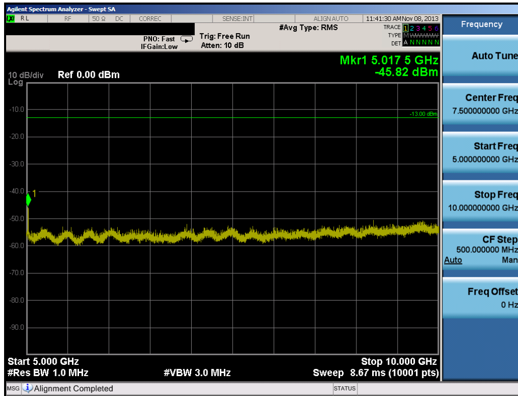
Plot 6-6. Conducted Spurious Plot (Cellular CDMA Mode – Ch. 384)
