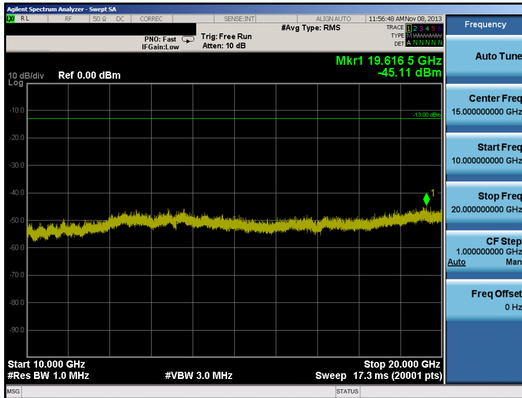
Plot 6-12. Conducted Spurious Plot (PCS CDMA Mode – Ch. 600)
