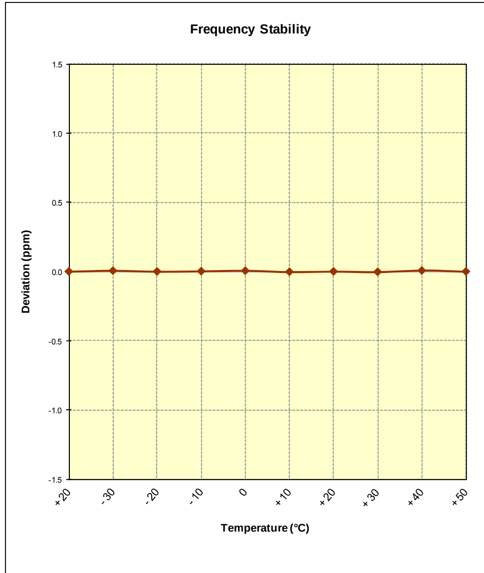
Figure 6-9. Frequency Stability Graph (PCS CDMA Mode – Ch. 600)
