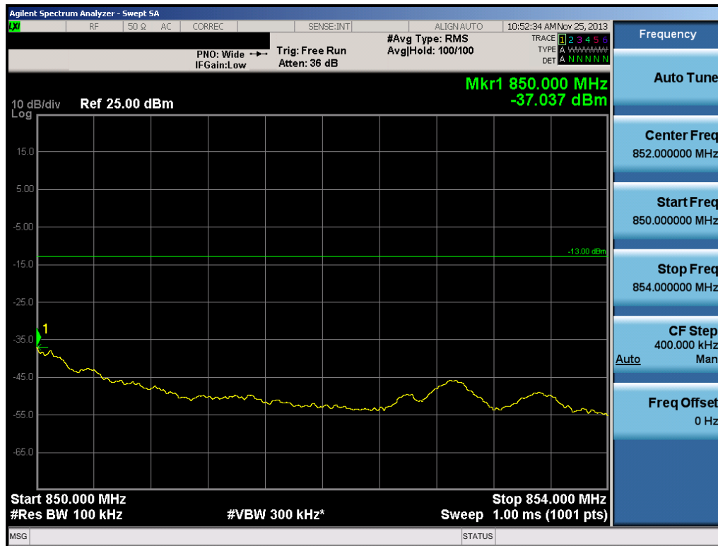
Plot 6-18. 4MHz Span Plot (Cellular CDMA Mode – Ch. 777)
