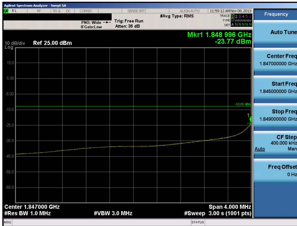
Plot 6-20. 4MHz Span Plot (PCS CDMA Mode – Ch. 25)
