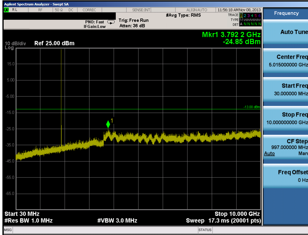
Plot 6-11. Conducted Spurious Plot (PCS CDMA Mode – Ch. 600)
