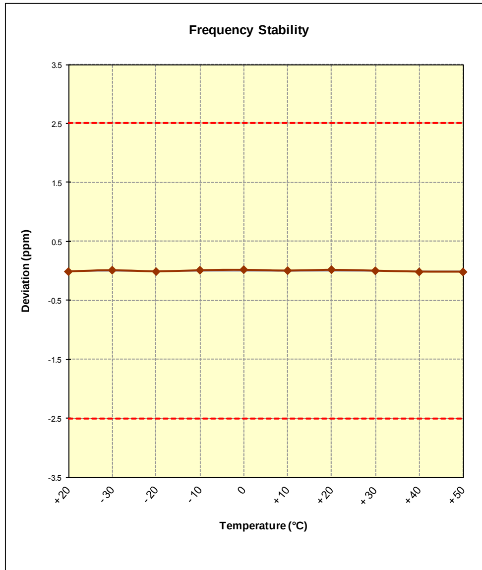
Figure 6-8. Frequency Stability Graph (Cellular CDMA Mode – Ch. 384)
