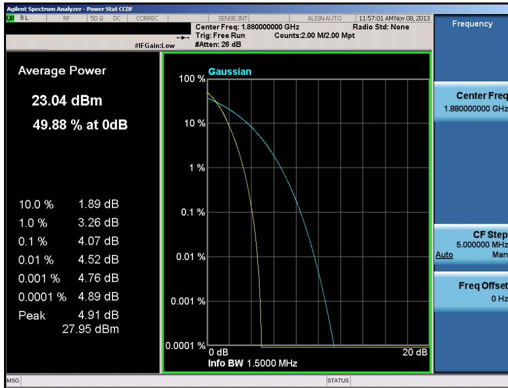
Plot 6-24. Peak-Average Ratio Plot (PCS CDMA Mode – Ch. 600)
