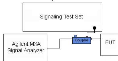
Figure 6-5. Test Instrument & Measurement Setup
