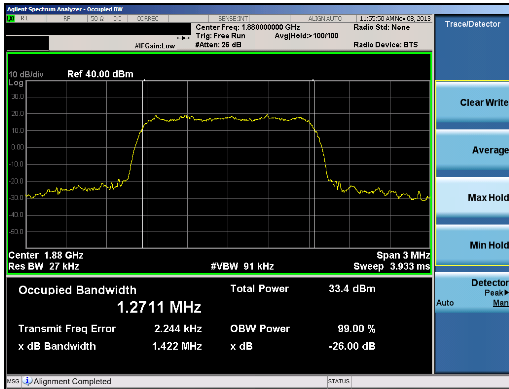
Plot 6-2. Occupied Bandwidth Plot (PCS CDMA Mode – Ch. 600)
