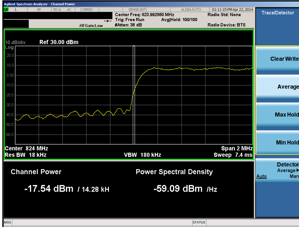
Plot 6-15. Band Edge Plot (Cellular CDMA Mode – Ch. 1013)
