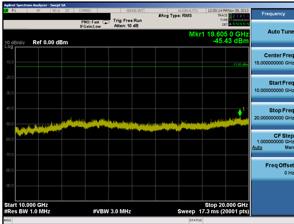
Plot 6-10. Conducted Spurious Plot (PCS CDMA Mode – Ch. 25)
