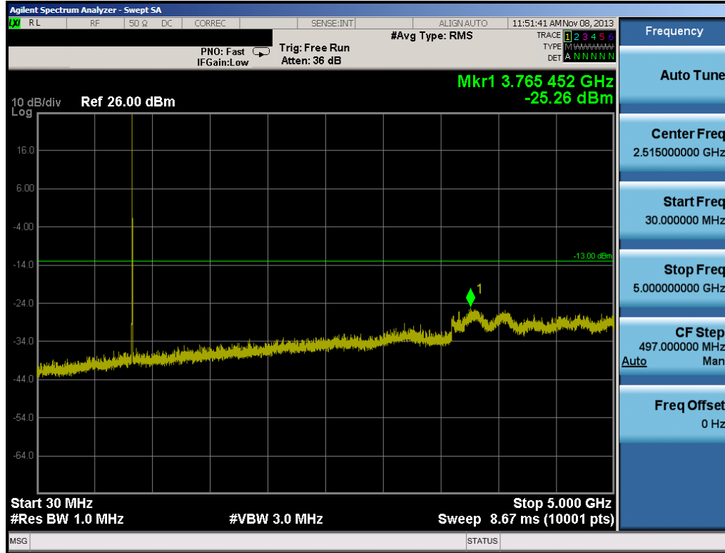
Plot 6-7. Conducted Spurious Plot (Cellular CDMA Mode – Ch. 777)
