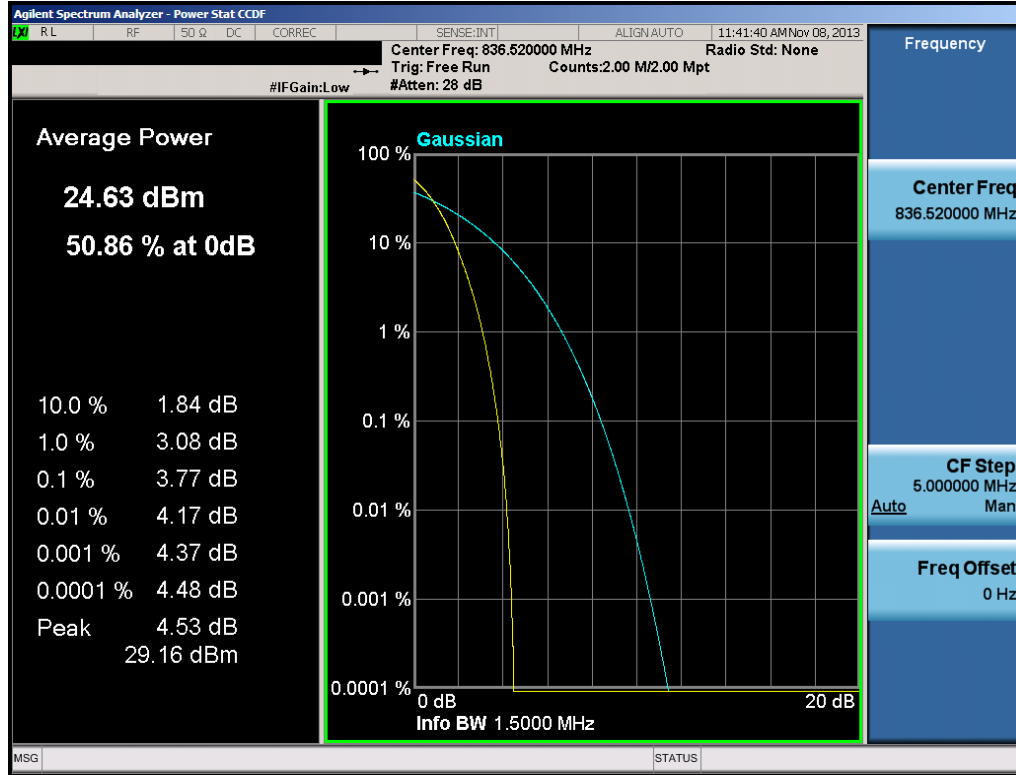
Plot 6-23. Peak-Average Ratio Plot (Cellular CDMA Mode – Ch. 384)
