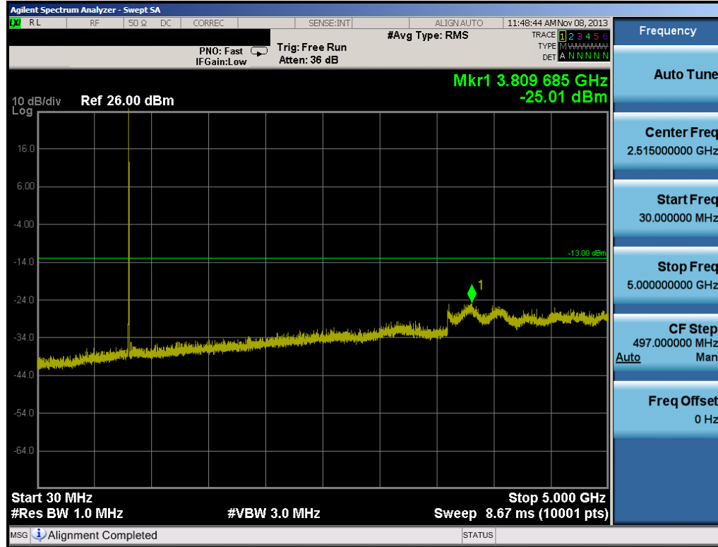
Plot 6-3. Conducted Spurious Plot (Cellular CDMA Mode – Ch. 1013)
