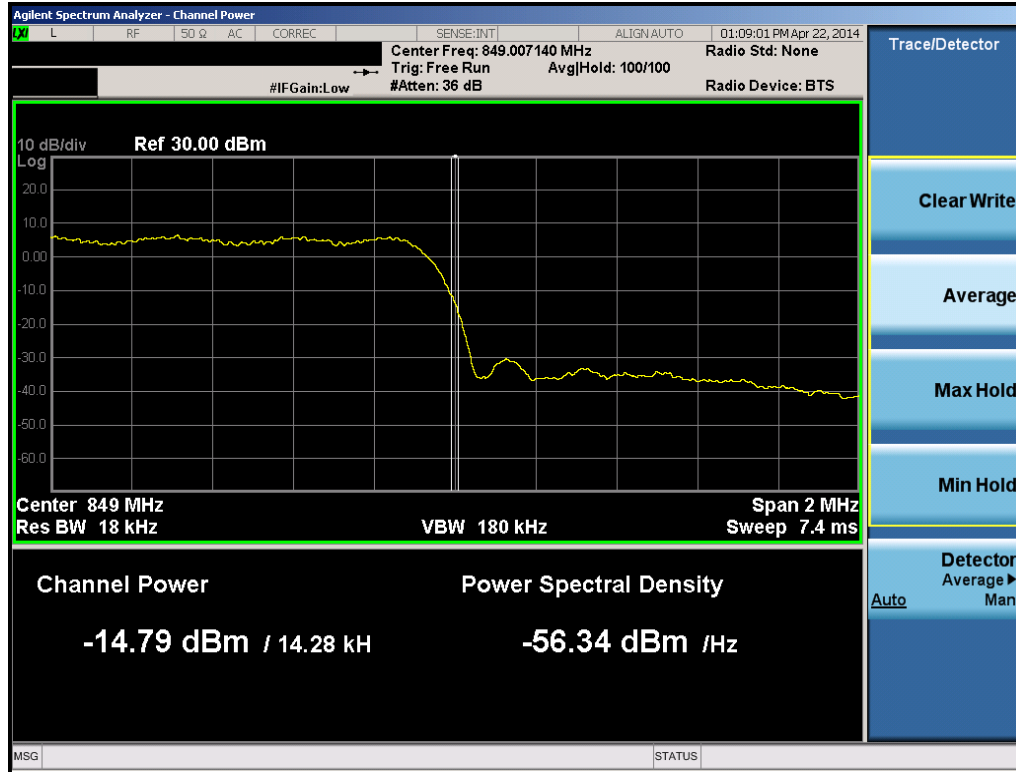
Plot 6-17. Band Edge Plot (Cellular CDMA Mode – Ch. 777)
