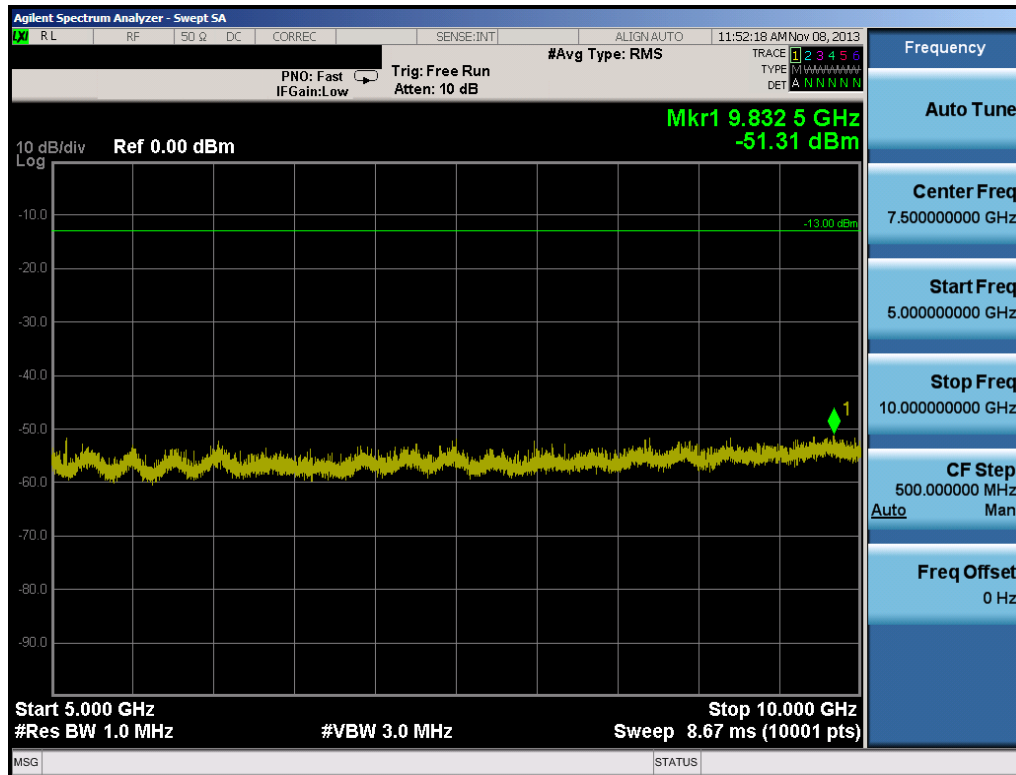
Plot 6-8. Conducted Spurious Plot (Cellular CDMA Mode – Ch. 777)
