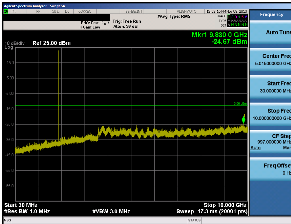
Plot 6-13. Conducted Spurious Plot (PCS CDMA Mode – Ch. 1175)
