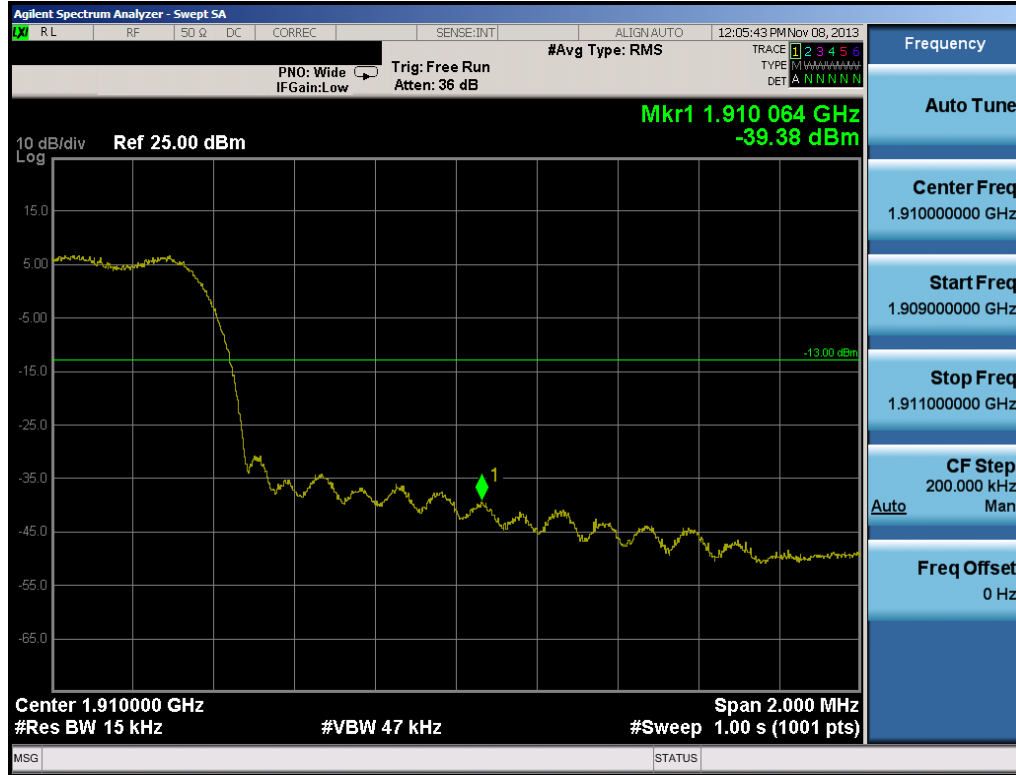
Plot 6-21. Band Edge Plot (PCS CDMA Mode – Ch. 1175)
