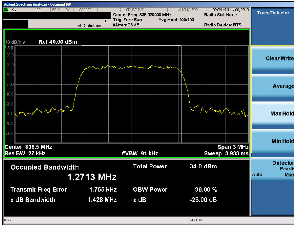
Plot 6-1. Occupied Bandwidth Plot (Cellular CDMA Mode – Ch. 384)
