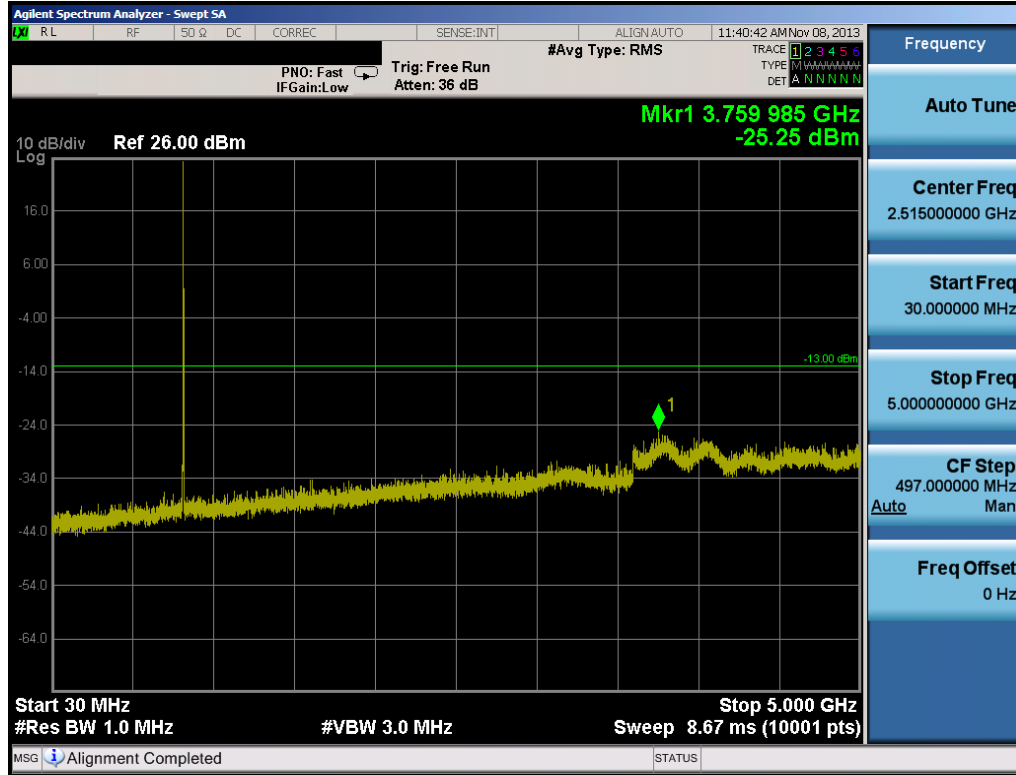
Plot 6-5. Conducted Spurious Plot (Cellular CDMA Mode – Ch. 384)
