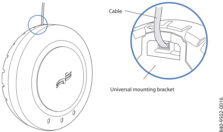
Figure 32. Step 8—Cable Placement
