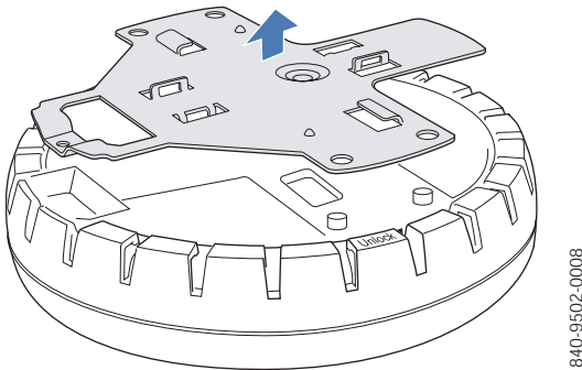
Figure 35. Step 1b—Removing the Bracket
