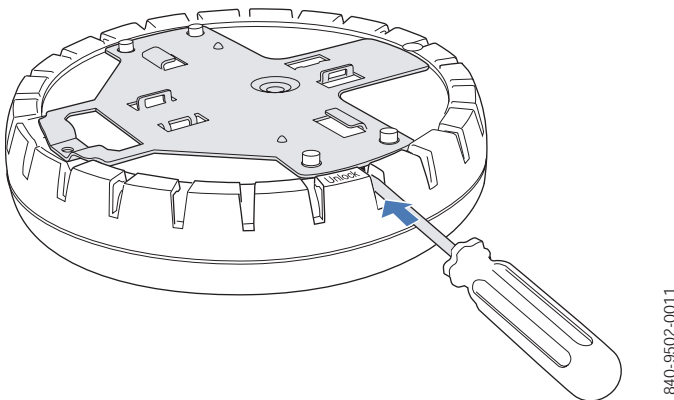
Figure 25. Step 1—Unlocking the Bracket
