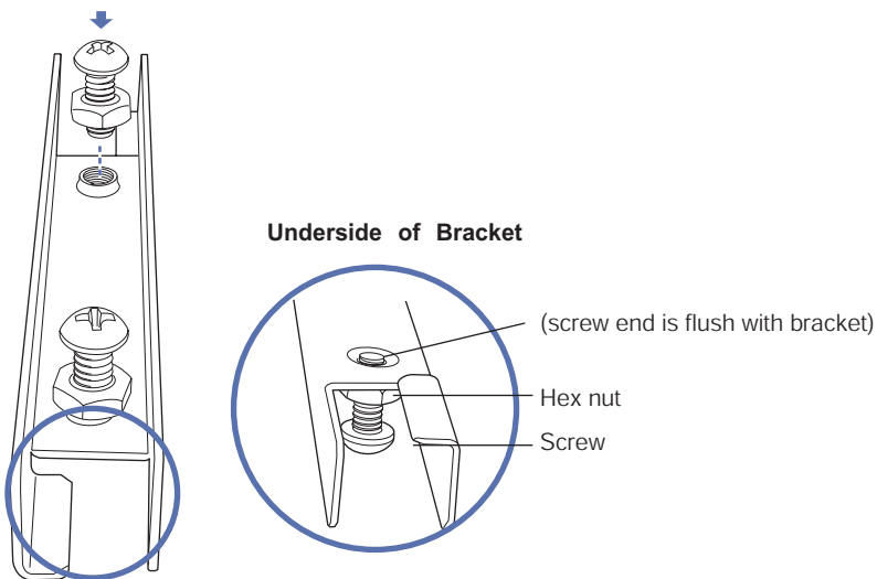
Figure 39. Step 3—Preparing the Mounting Bracket
