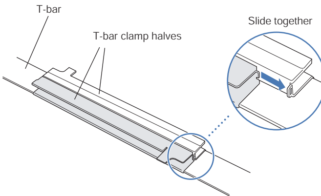
Figure 10. Step 4—Installing a T-bar Clamp
