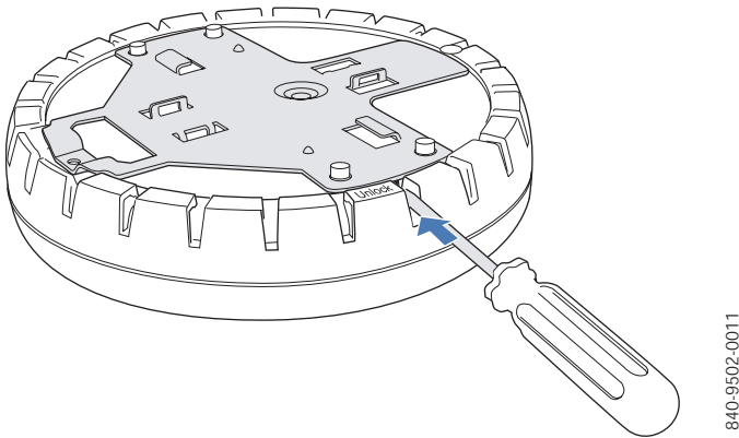
Figure 11. Step 5—Unlocking the Bracket
