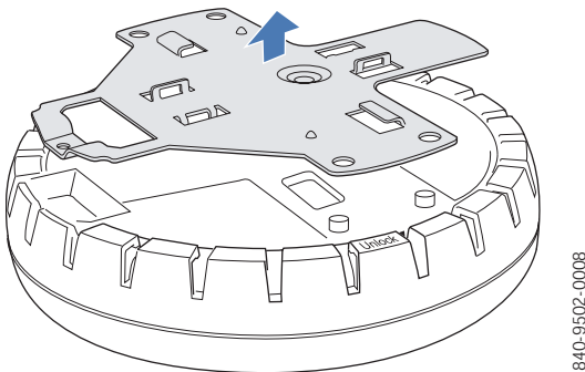
Figure 12. Step 6—Removing the Bracket
