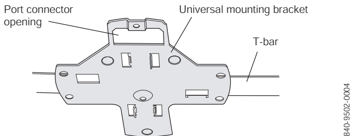
Figure 22. Step 6—Bottom View
