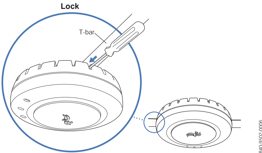
Figure 24. Step 10—Locking the Bracket
