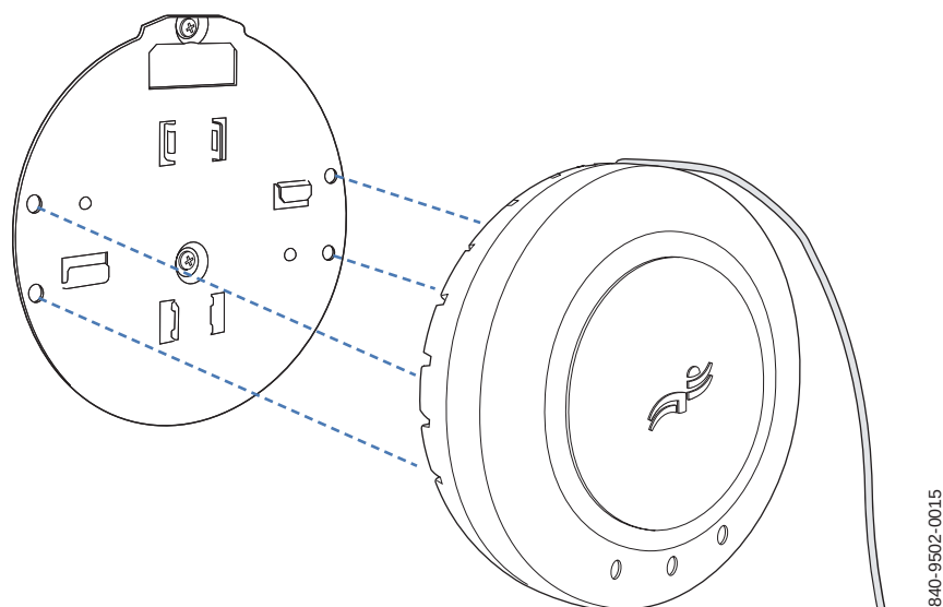
Figure 29. Steps 7 and 8—bracket alignment
