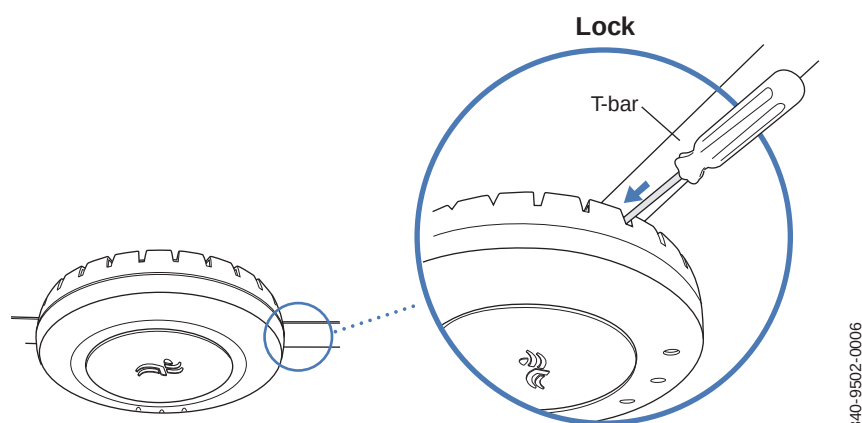
Figure 23. Step 9—locking the bracket
