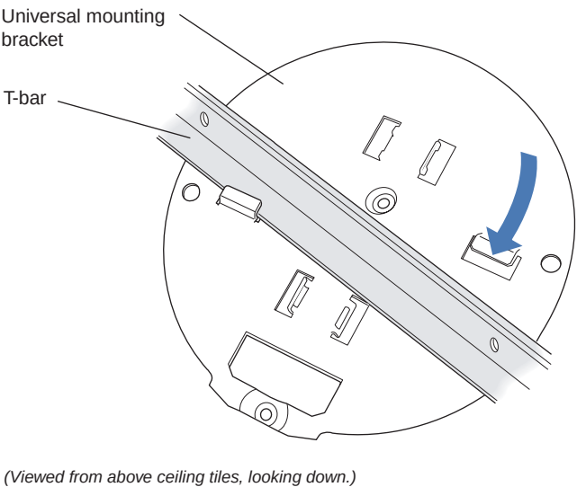
Figure 14. Step 6—top view for 14.2-mm (9/16-inch) T-bar
