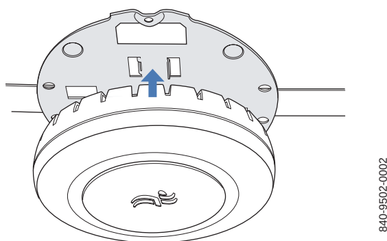
Figure 16. Step 9—placing the MP access point on the bracket
