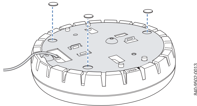
Figure 35. Steps 2 and 3—installing the rubber feet
