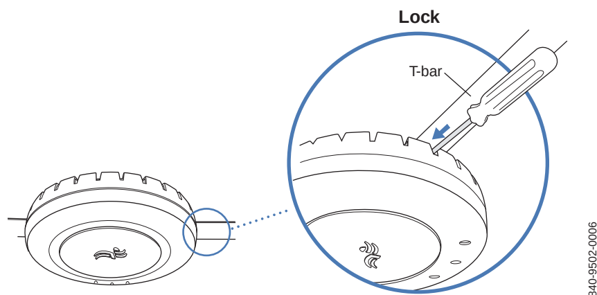
Figure 17. Step 10—locking the bracket
