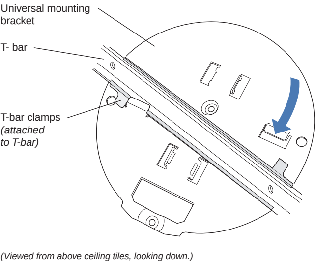
Figure 15. Step 6—bottom view
