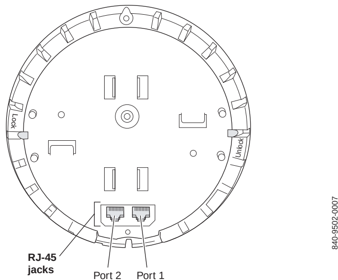
Figure 2. MP access point—bottom view
