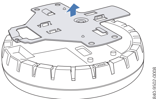
Figure 24. Step 2—Removing the Bracket
