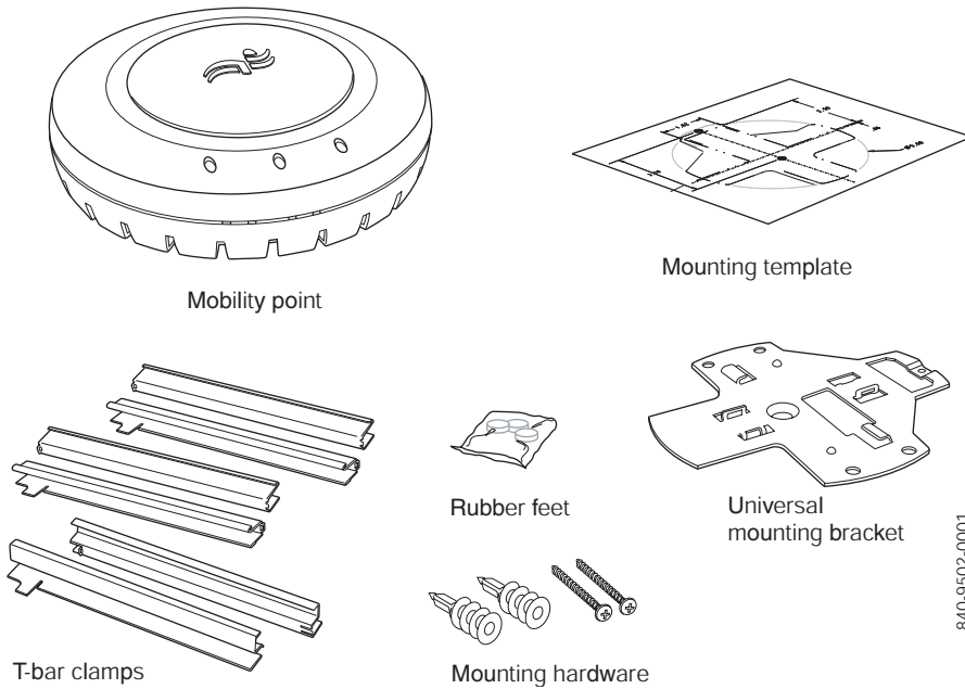
Figure 5. MP-372 Shipping Carton Contents
