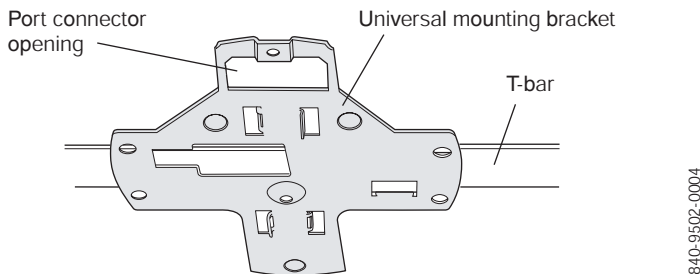
Figure 19. Step 6—Bottom View
