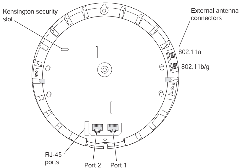
Figure 2. MP Access Point Model MP-372—Bottom View
