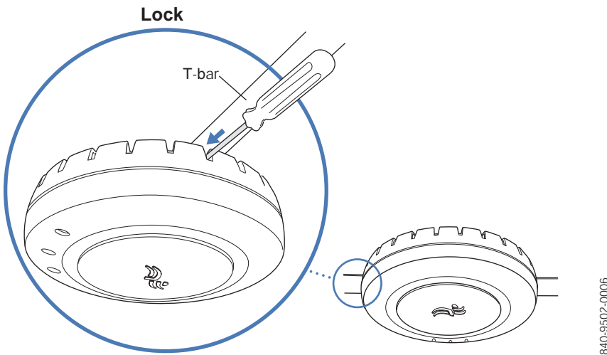
Figure 13. Step 11—Locking the Bracket
