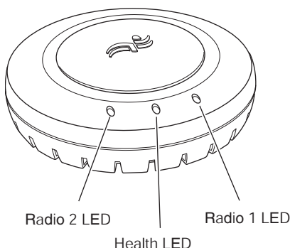
Figure 4. Health and Radio LEDs—MP-372
