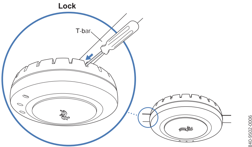
Figure 21. Step 10—Locking the Bracket
