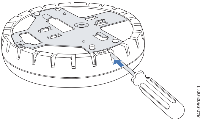
Figure 26. Step 3—Unlocking the Bracket
