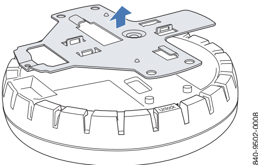
Figure 27. Step 4—Removing the Bracket
