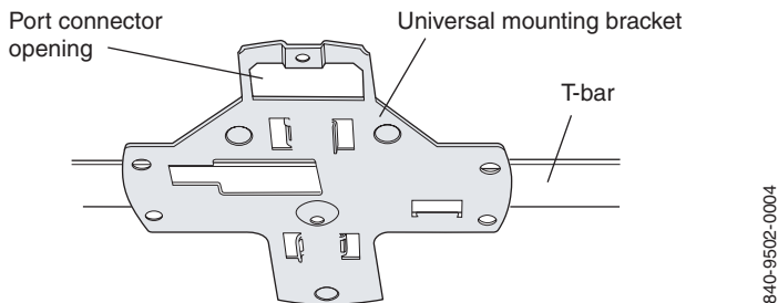
Figure 19. Step 6—Bottom View
