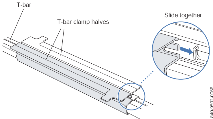
Figure 15. Step 3—Installing the T-bar Clamp for a 15.9-mm (5/8-inch) T-bar
