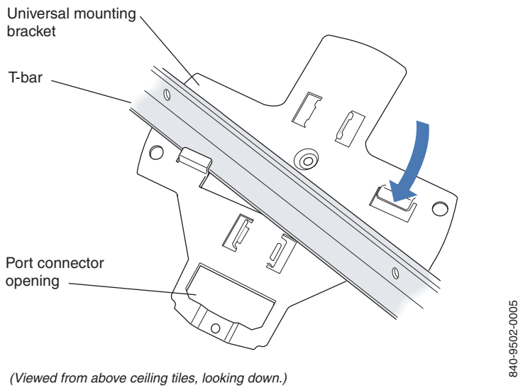
Figure 10. Step 7—Top View
