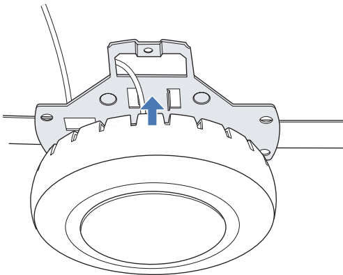
Figure 12. Step 10—Placing the MP Access Point on the Bracket
