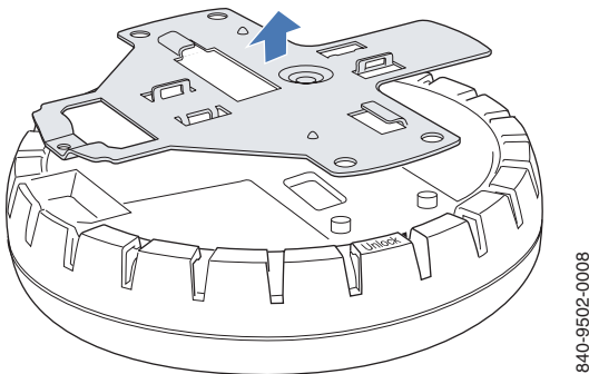
Figure 9. Step 6—Removing the Bracket
