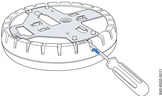
Figure 22. Step 1—Unlocking the Bracket
