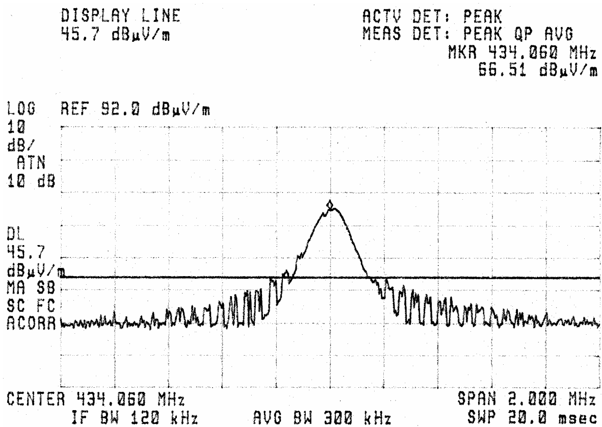
Figure 5.1 Occupied Bandwidth
