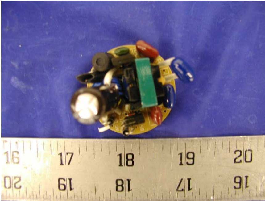
EUT – EL8us-15 Component View
