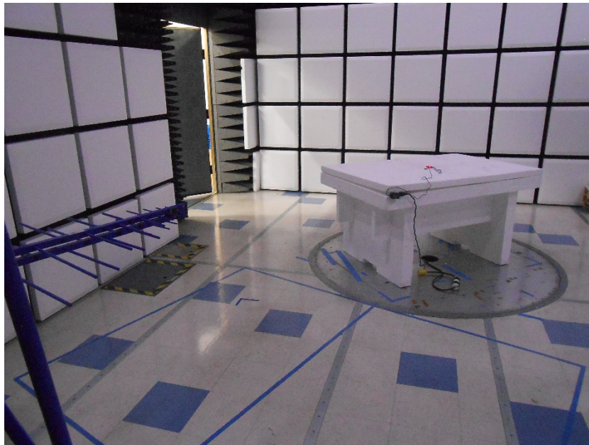
Radiated < 1GHz
