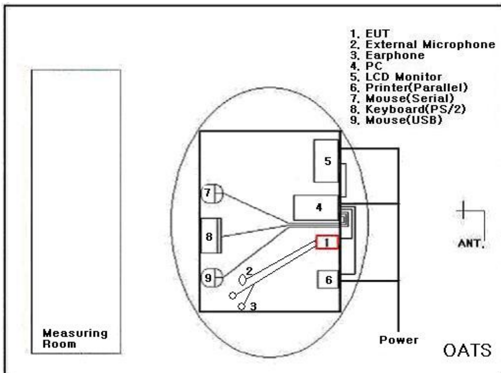
Radiated Emissions
