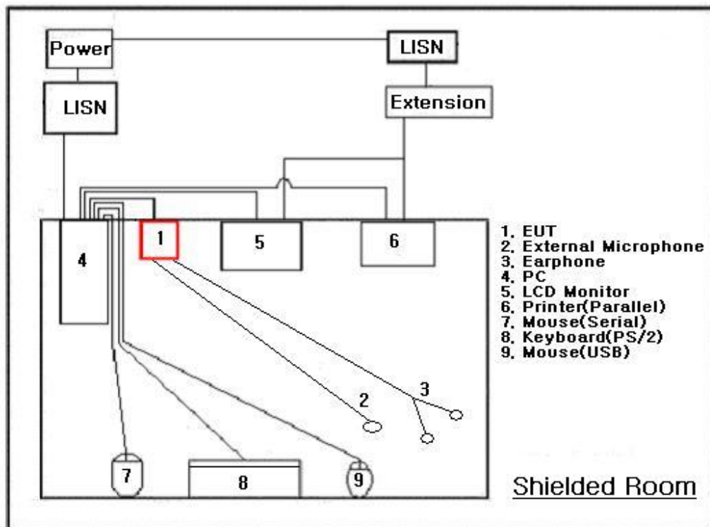
Conducted Emissions
