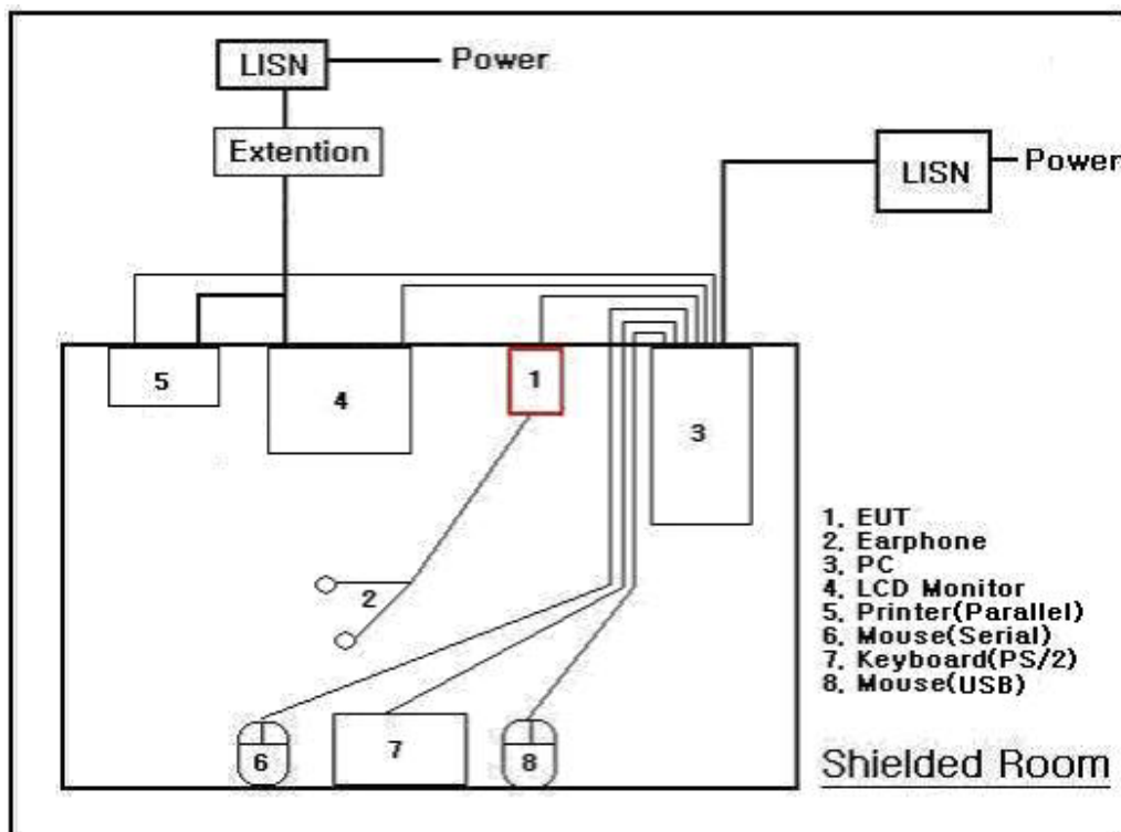
Conducted Emissions
