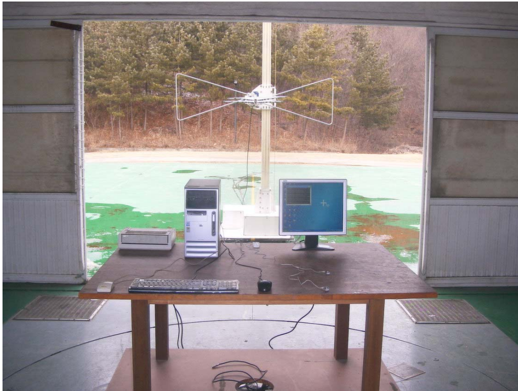
Radiated Emissions (30MHz-1GHz)-Front View(Files read/write mode)
