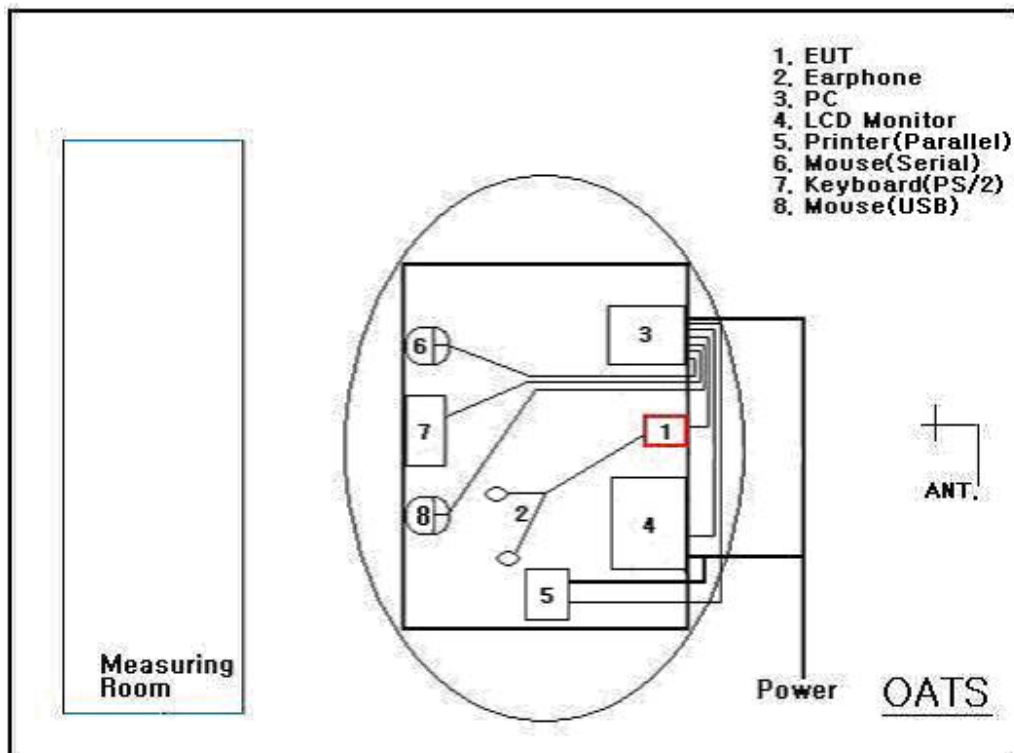
Radiated Emissions
