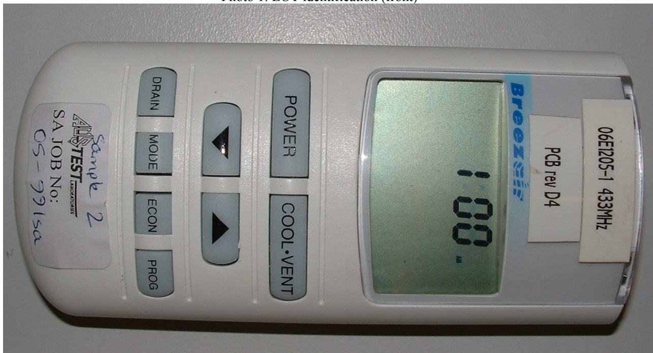
Photo 1: EUT identification (front)
