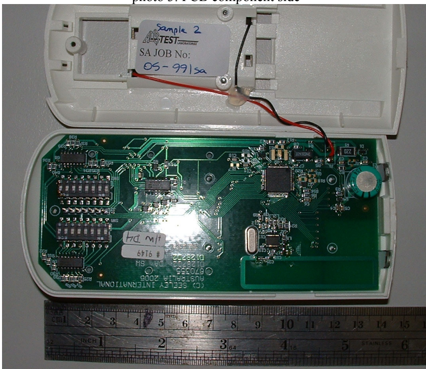
photo 3: PCB component side
