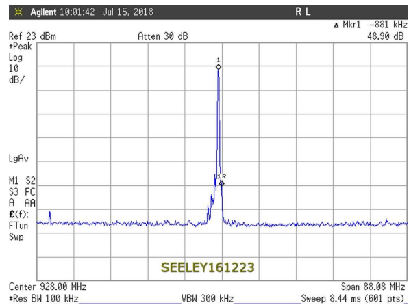
928MHz – High Channel
