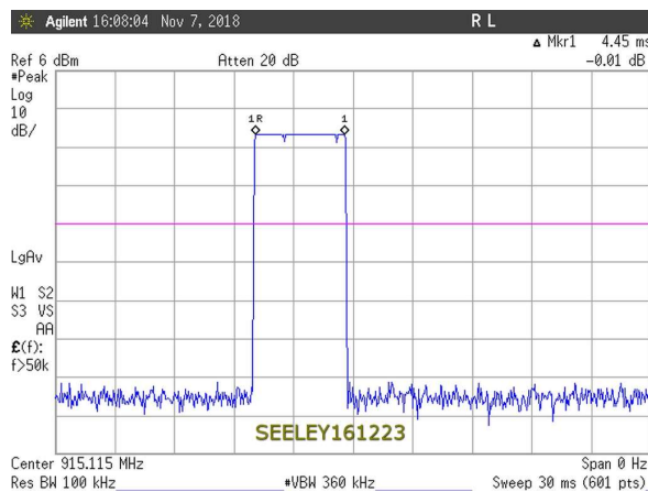
Time of Occupancy - Low Channel
