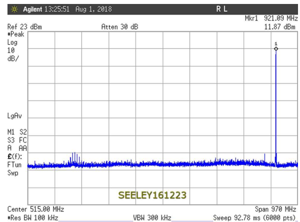
30MHz to 1000MHz – Middle Channel
