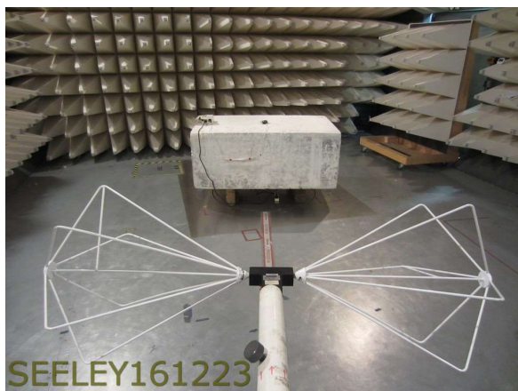
Radiated Emissions Below 1GHz - Wireless Receiver
