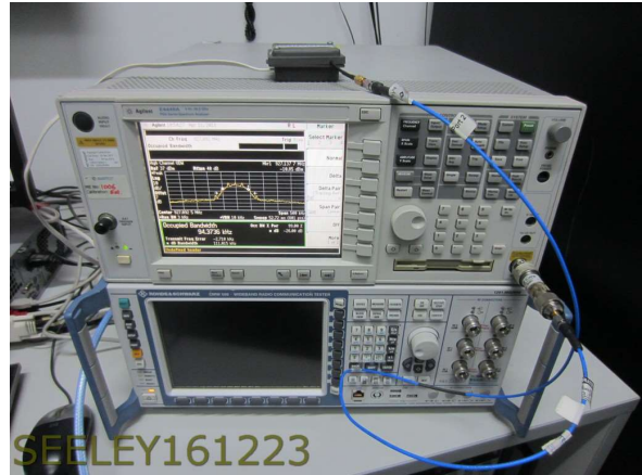
Antenna Port Tests – Wireless Receiver
