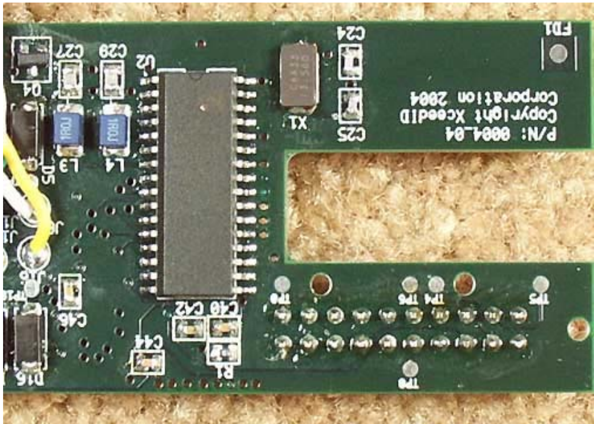
Base Front PCB Close-up 4
