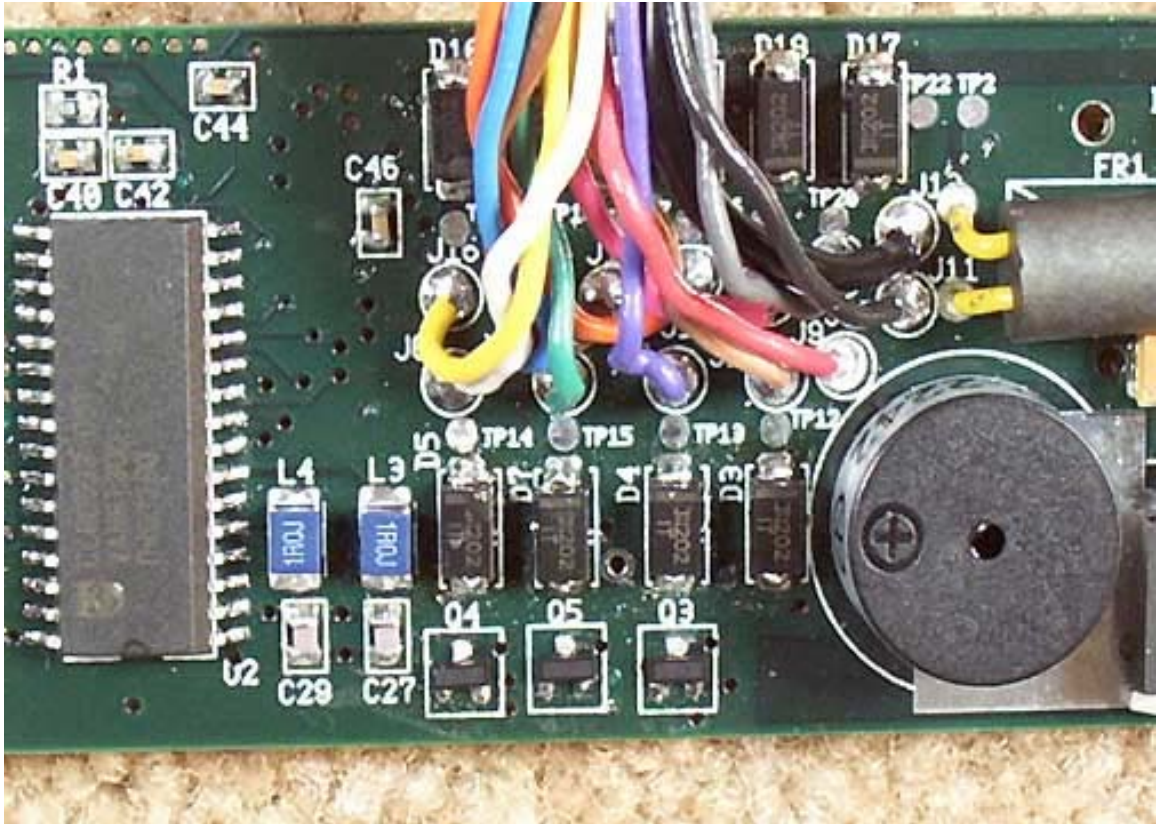
Base Front PCB Close-up 3
