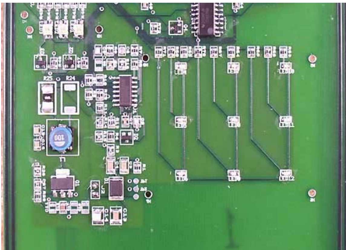
21xx Front Antenna PCB Close-up 2
