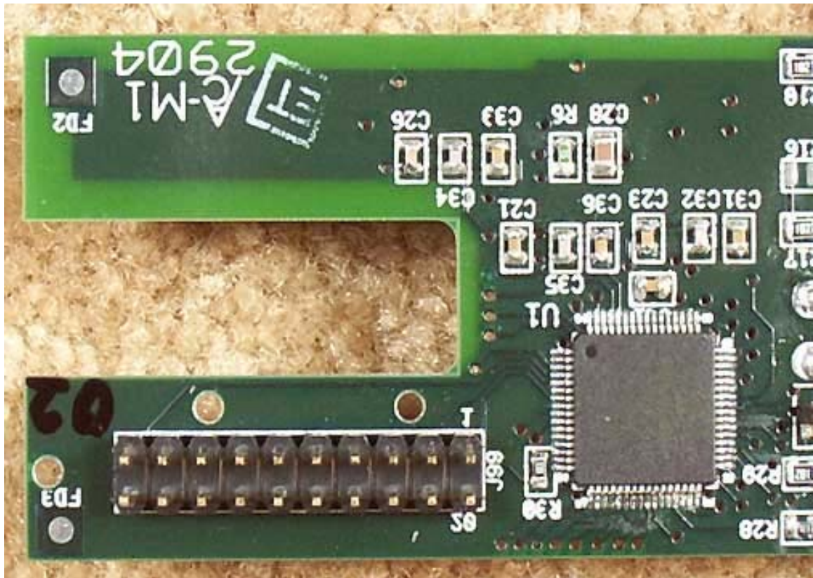
Base PCB Back Close-up 1
