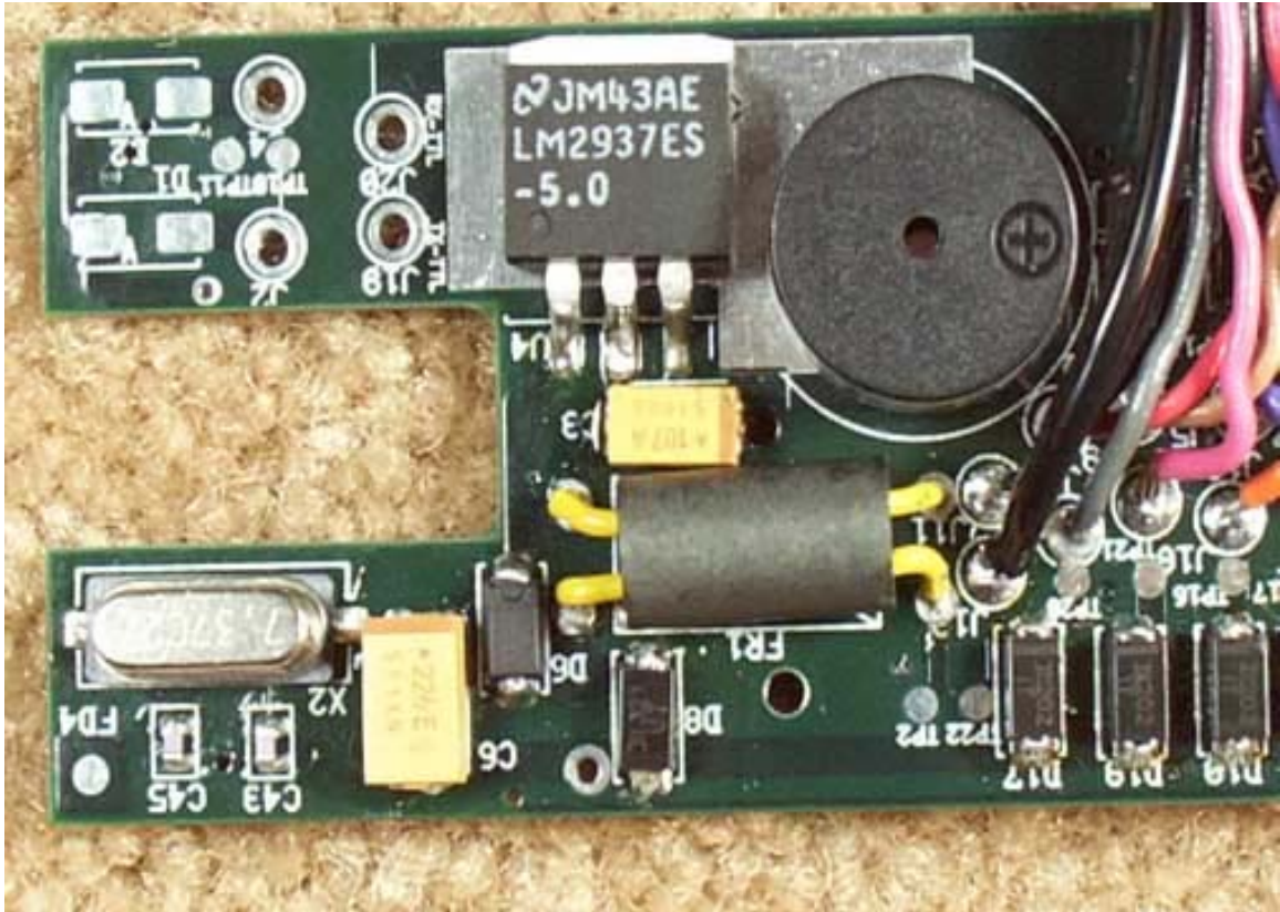
Base Front PCB Close-up 1
