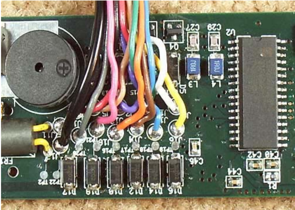
Base Front PCB Close-up 2
