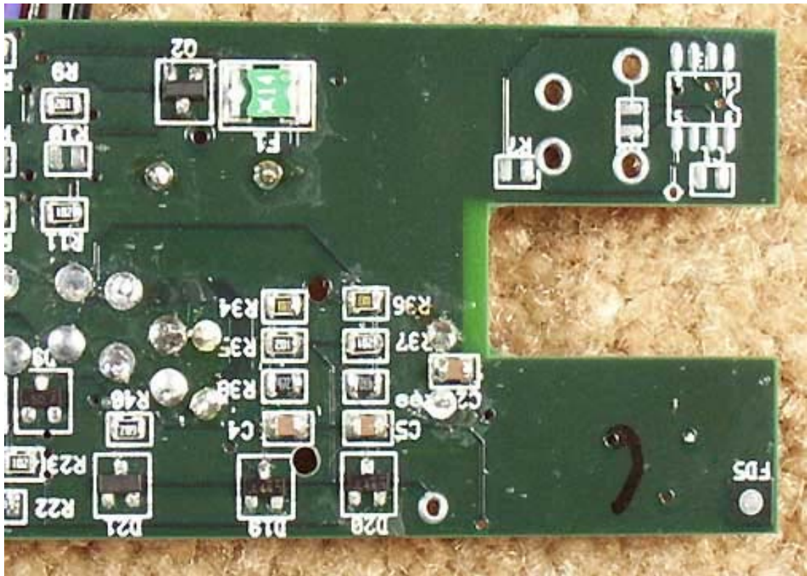
Base PCB Back Close-up 3
