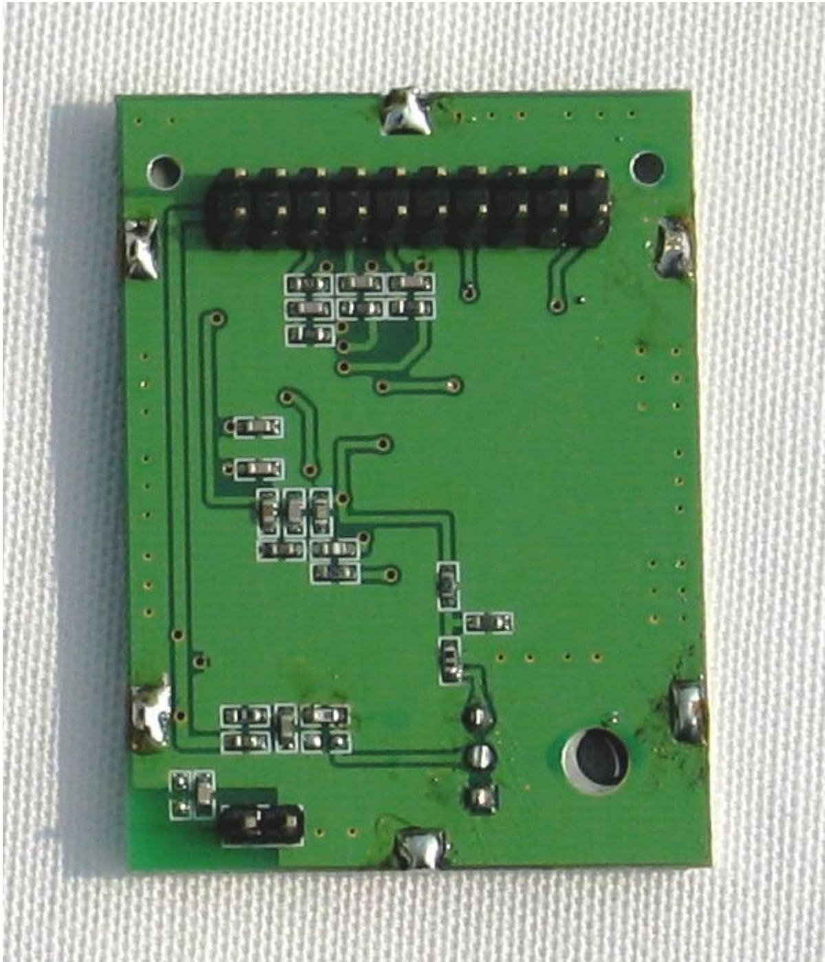
Underside of TX Module Board
