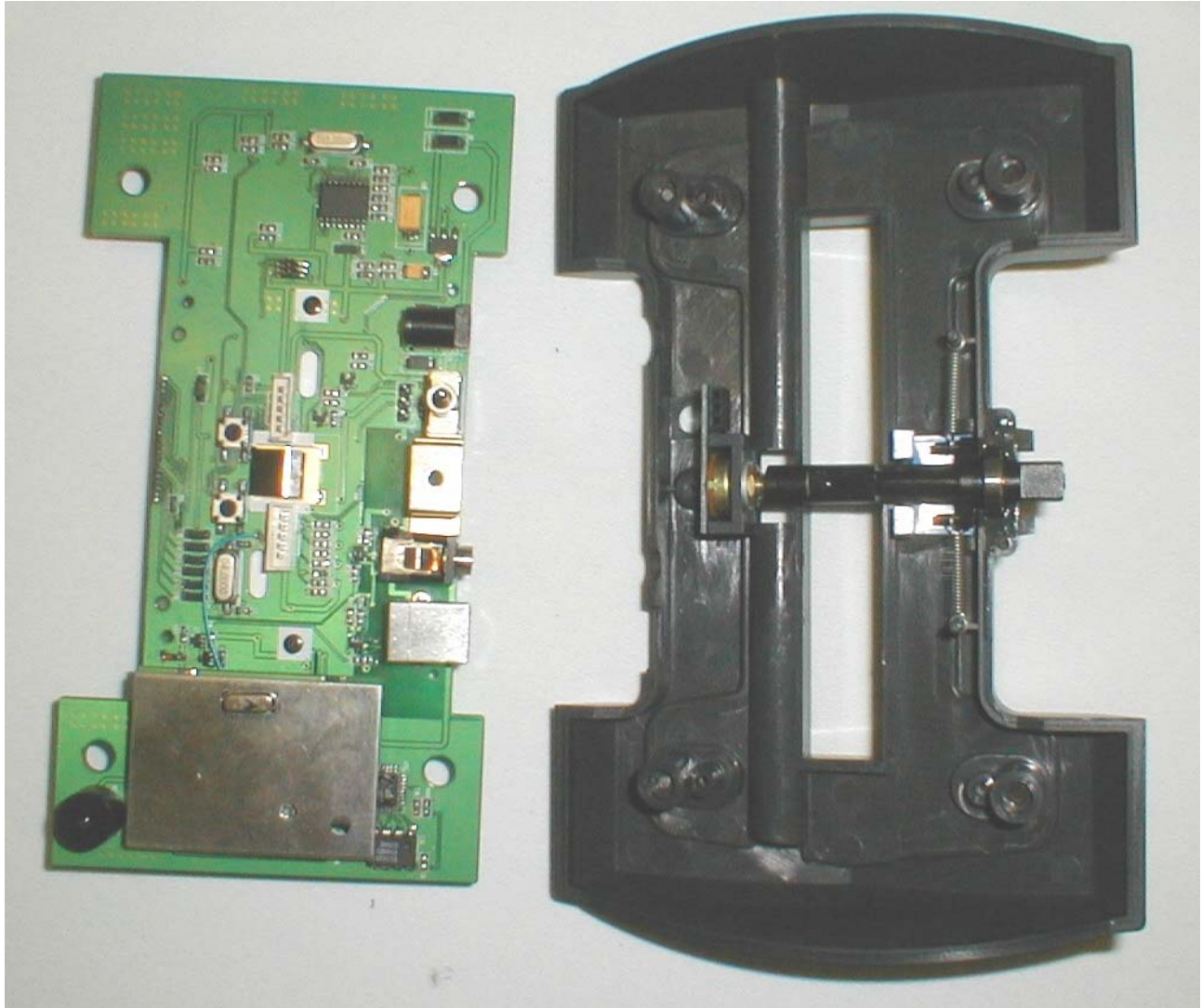
Main PCB Removed From Housing
