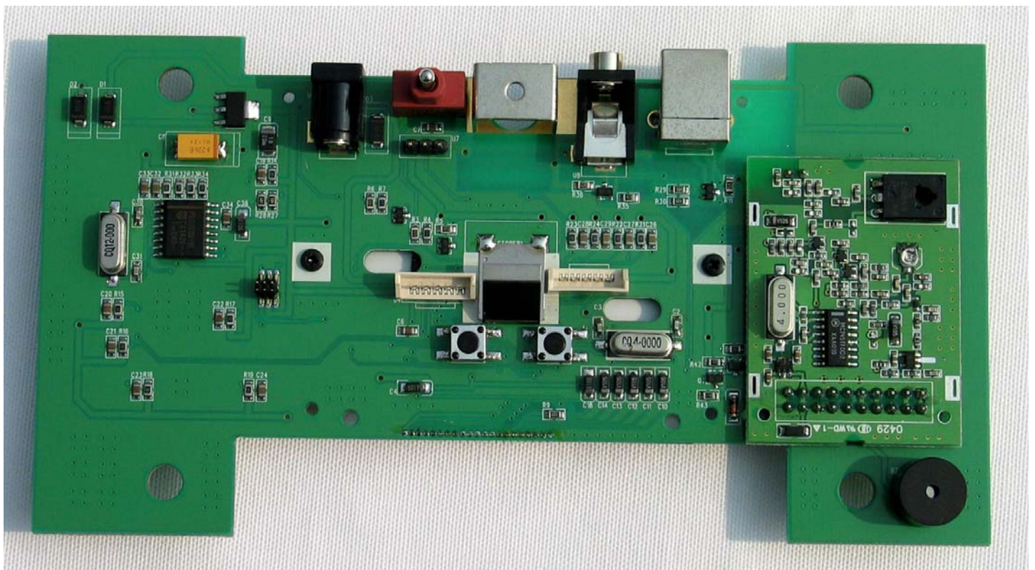
Shield Removed
