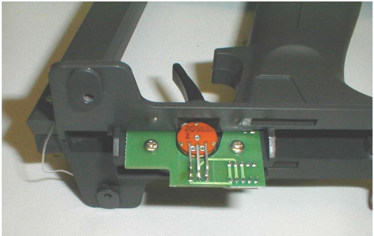
Trigger PCB
