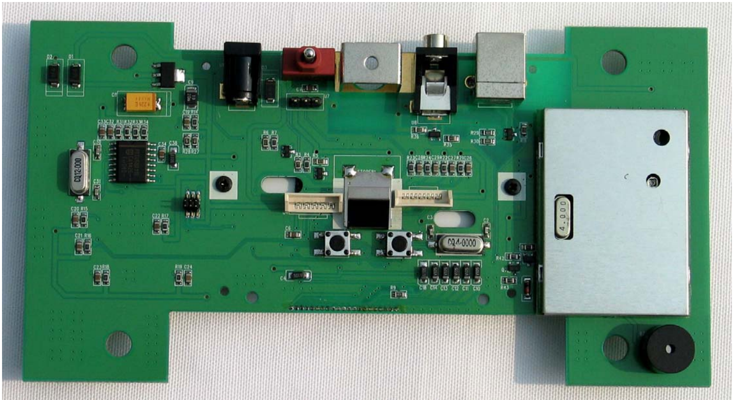
Shield Removed
