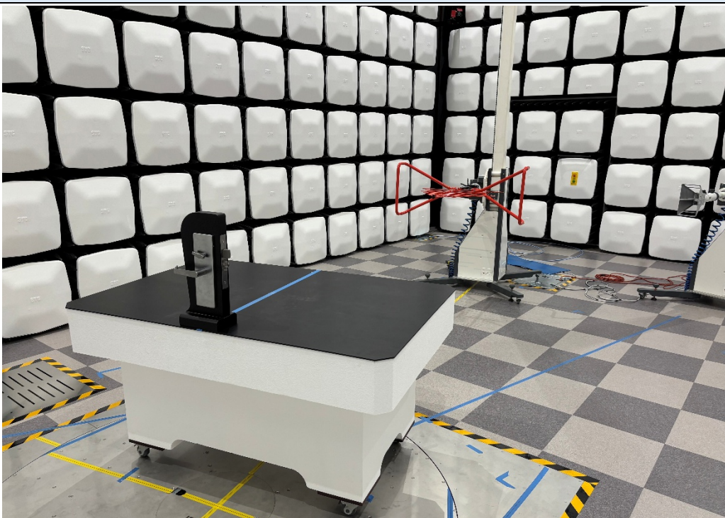
30 MHz – 1GHz
