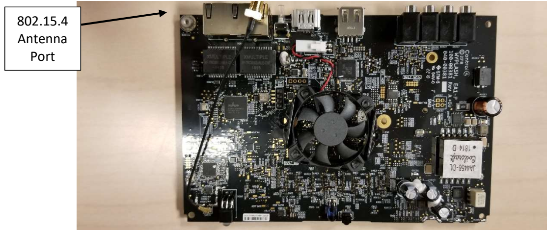
Photograph 1 – Top View of the PCB
