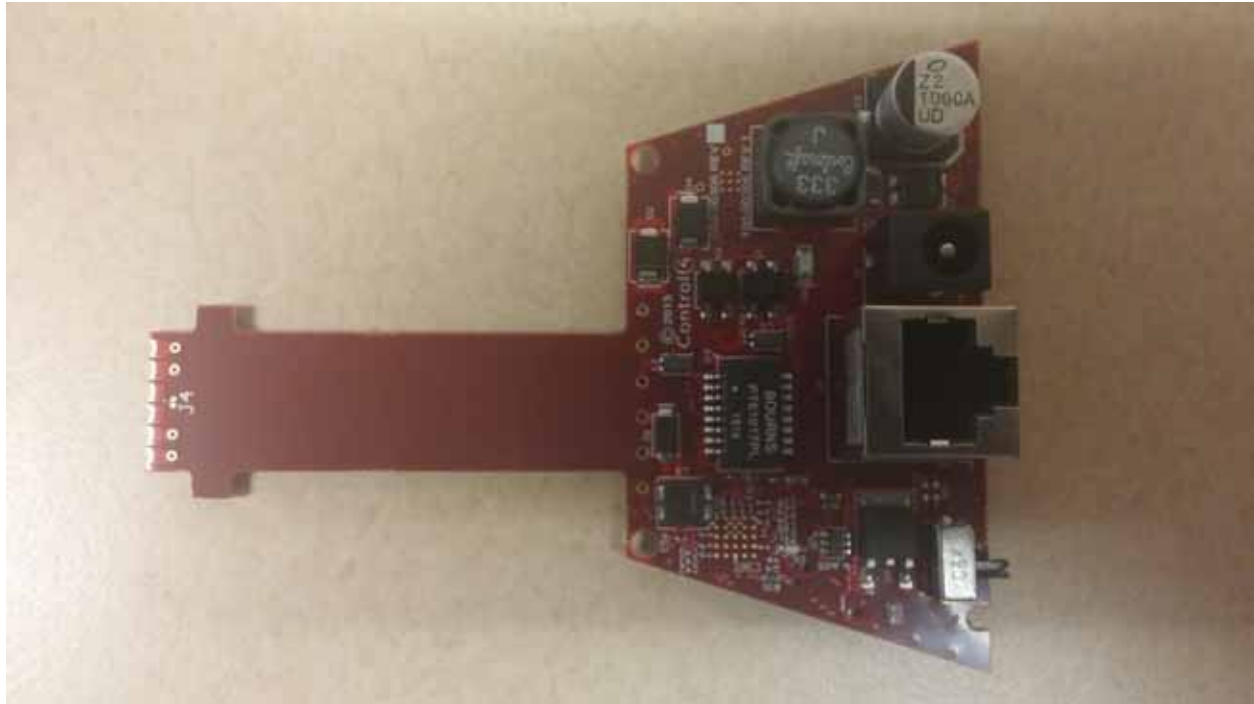
Photograph 16 – View of the Back Side of the Base PCB
