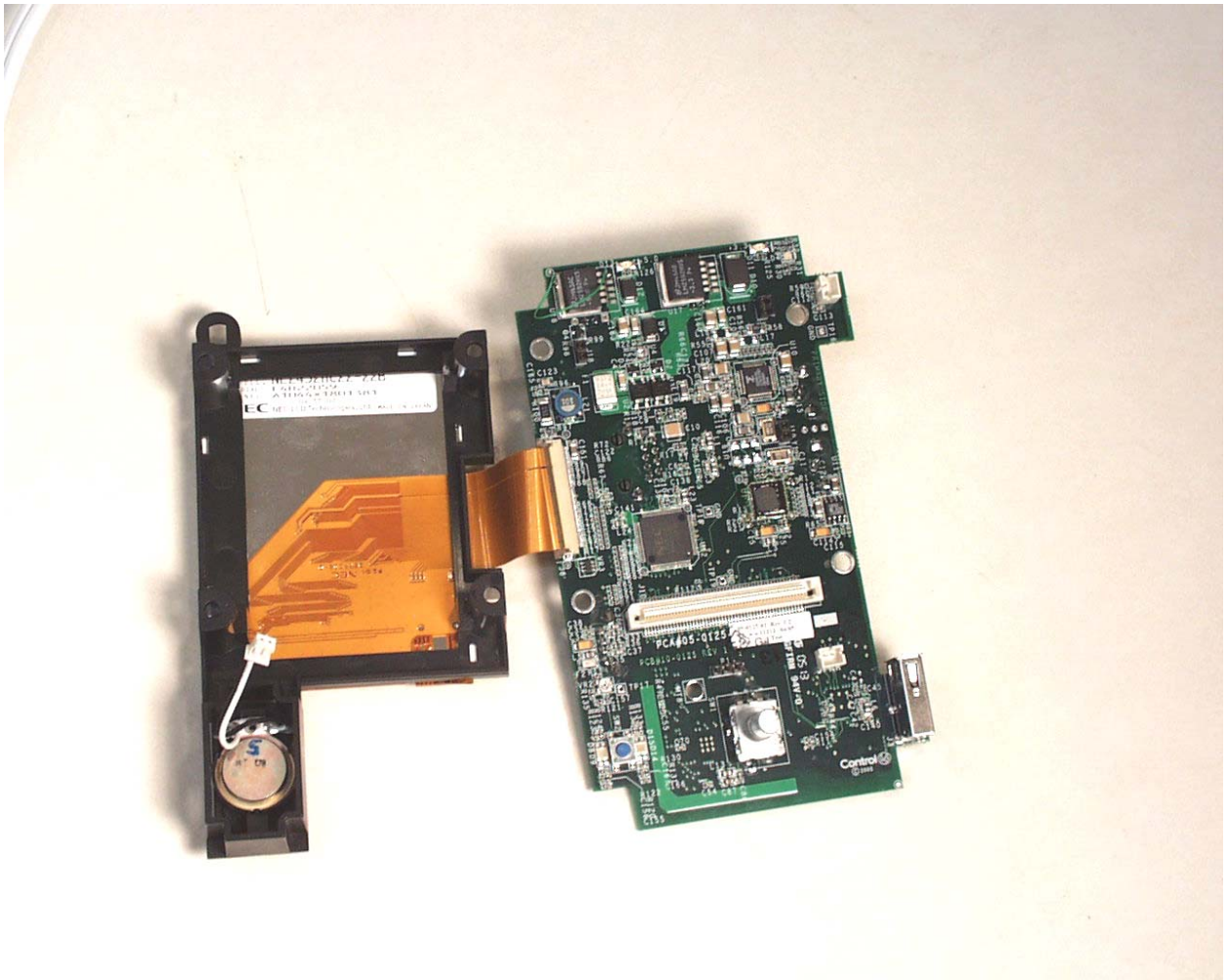
Top View of the Main PCB of the EUT and Back Side of the Display Module
