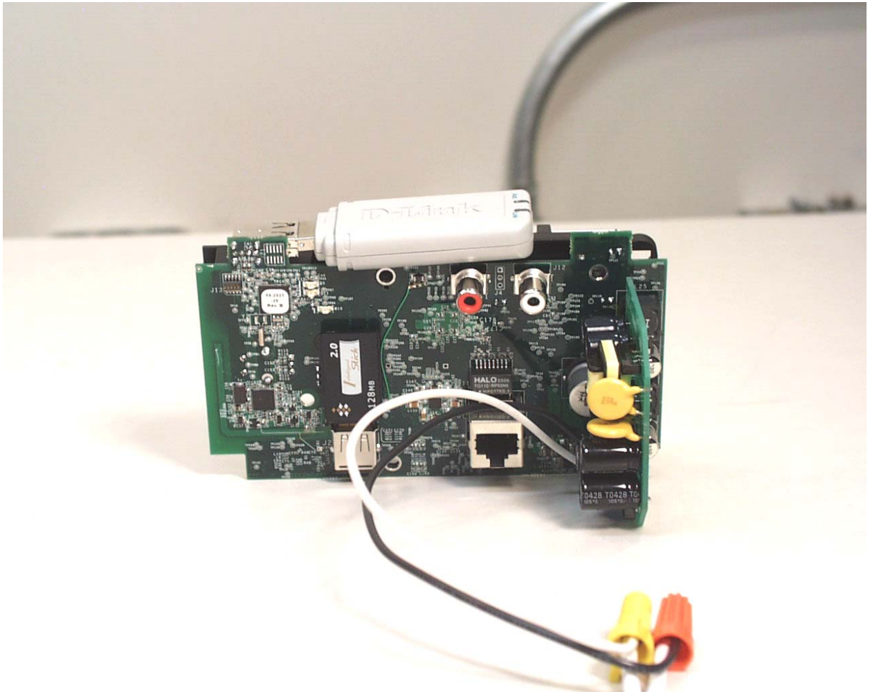
Back View of the EUT with the USB Devices Installed
