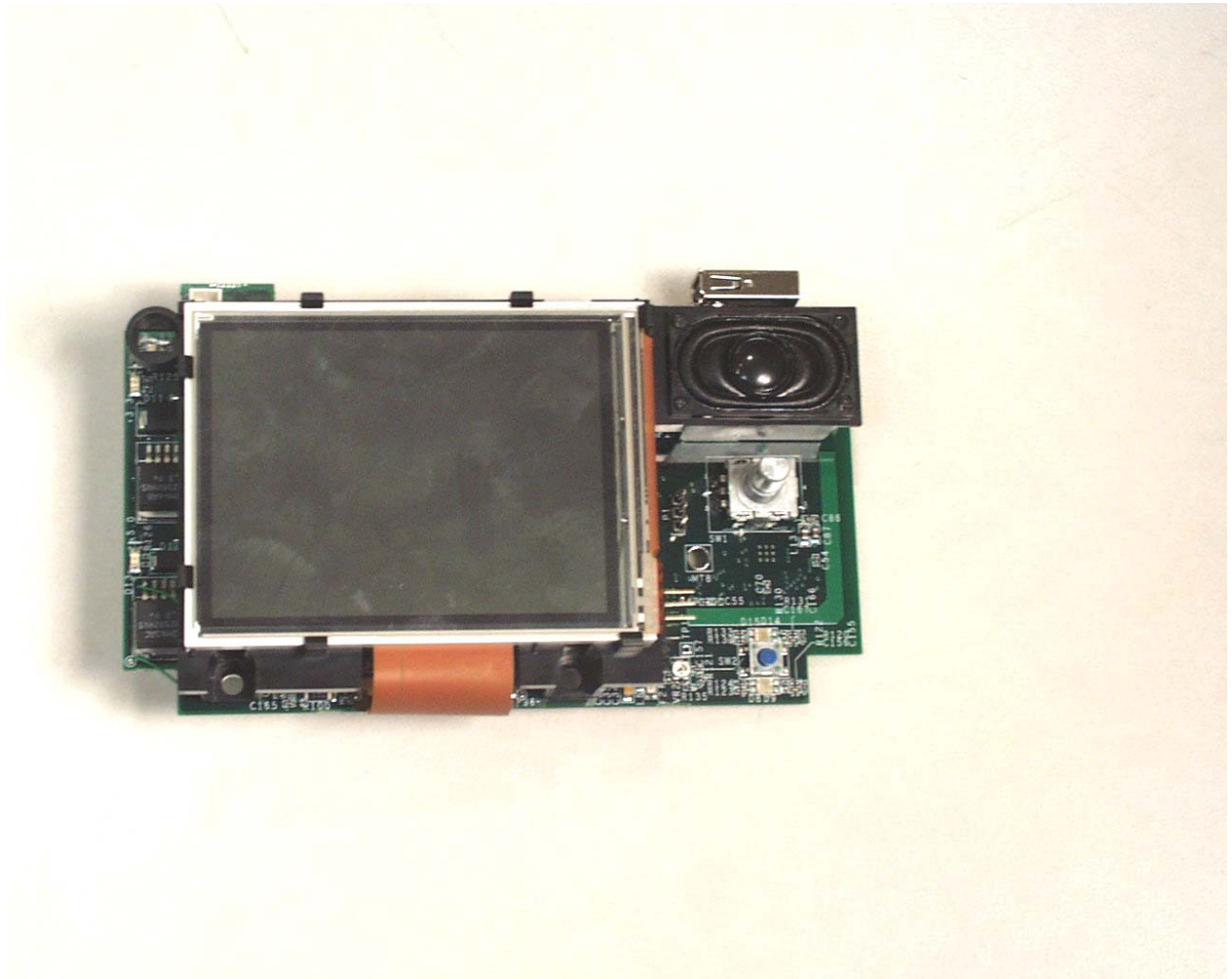
Front View of the EUT without the USB Devices Installed
