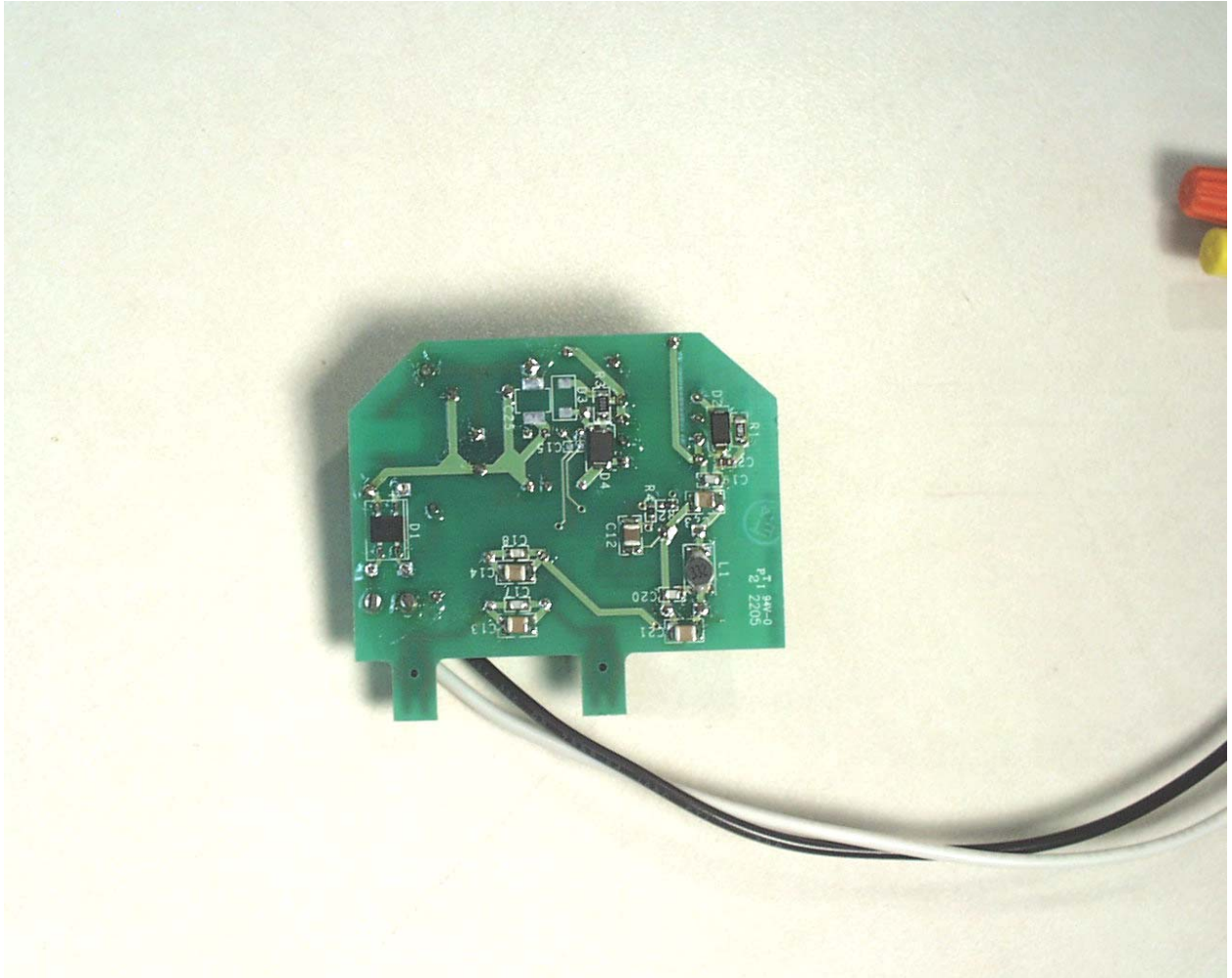
View of the Trace Side of the Power Supply Module
