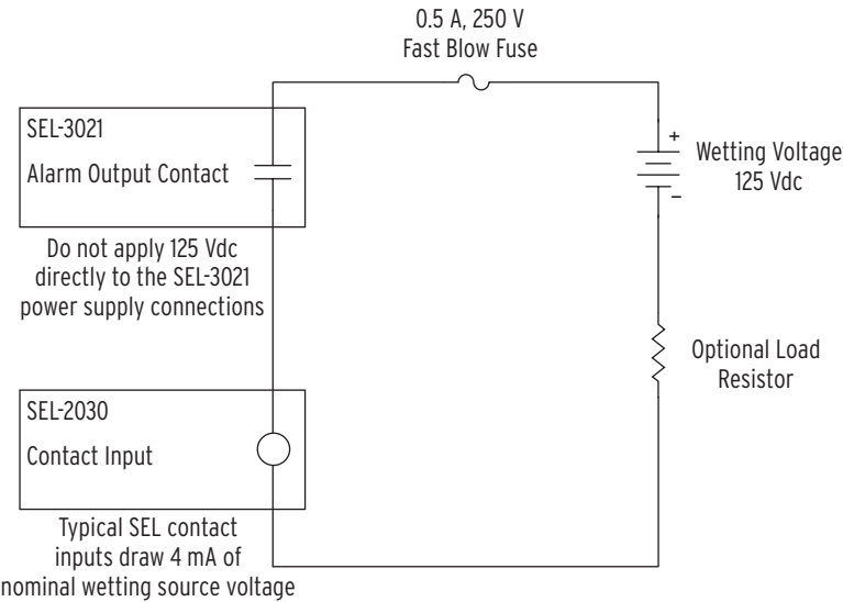
Figure 1.4 Typical Alarm Output Installation
