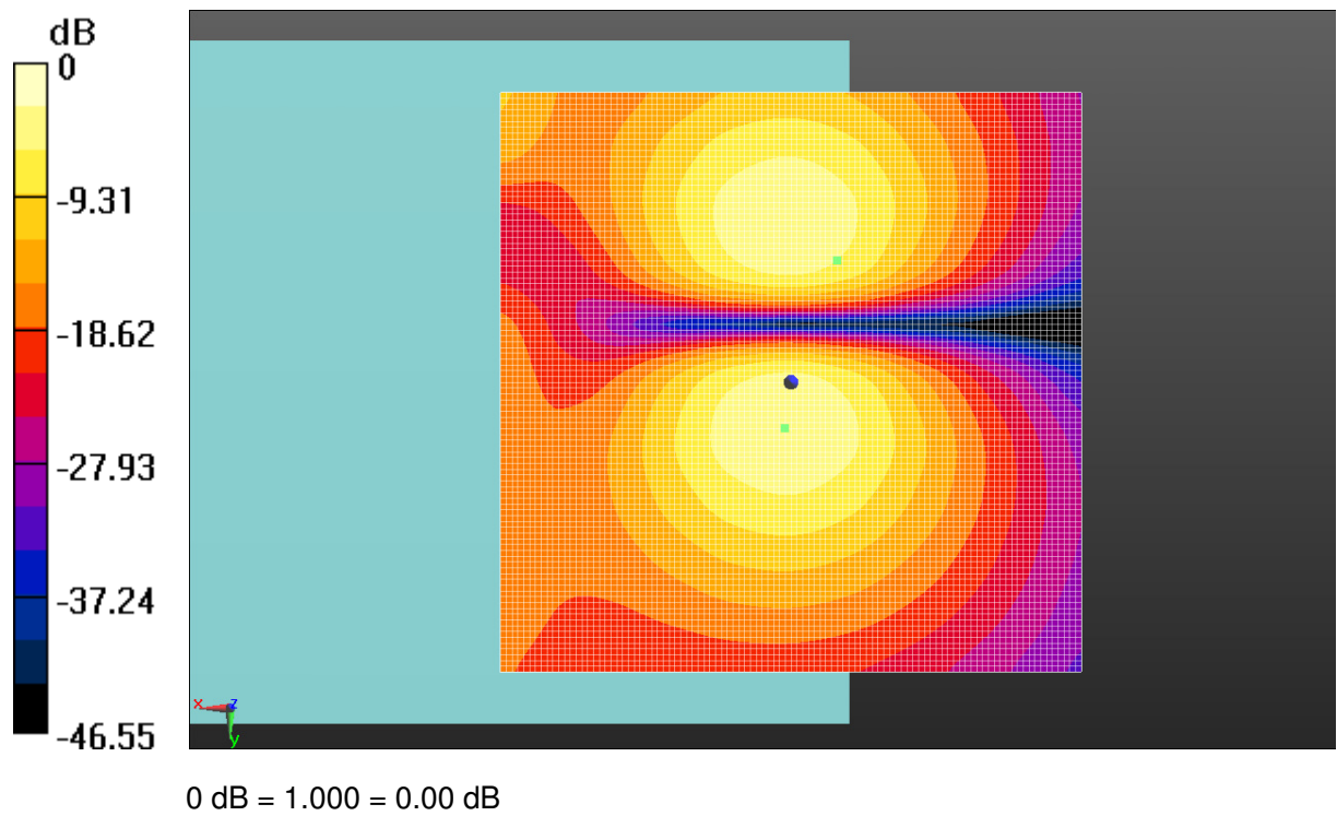
Fig B.1 T-Coil GSM 850
