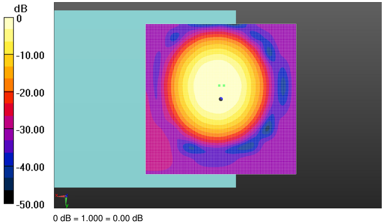
Fig B.10 T-Coil WCDMA 1900
