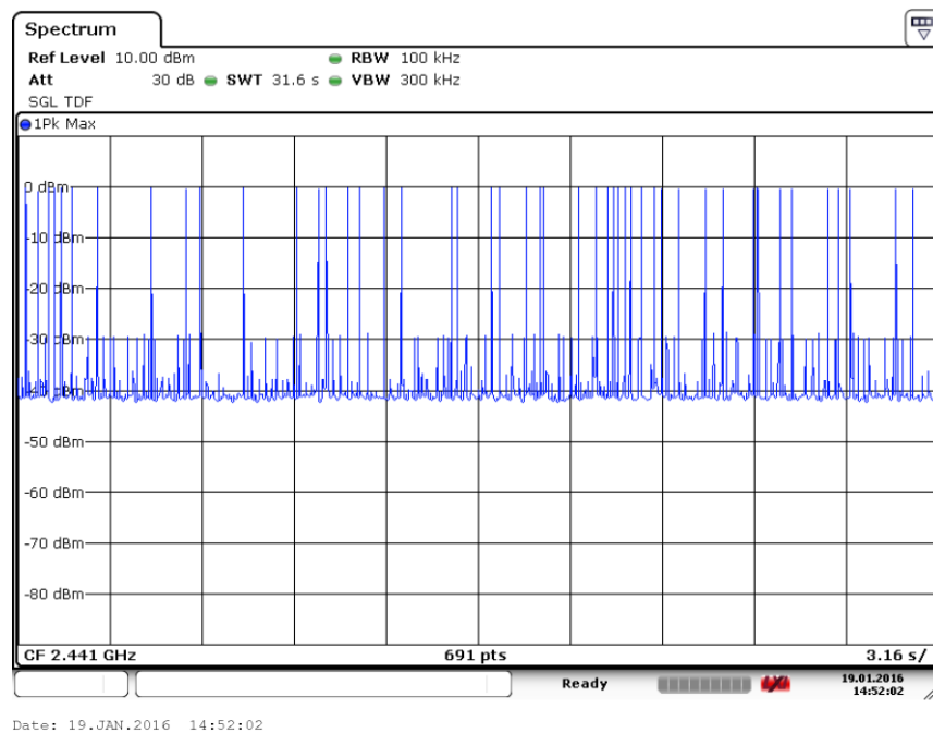
Fig. 84 Number of Transmissions ( \pi/4 DQPSK, Ch39)
