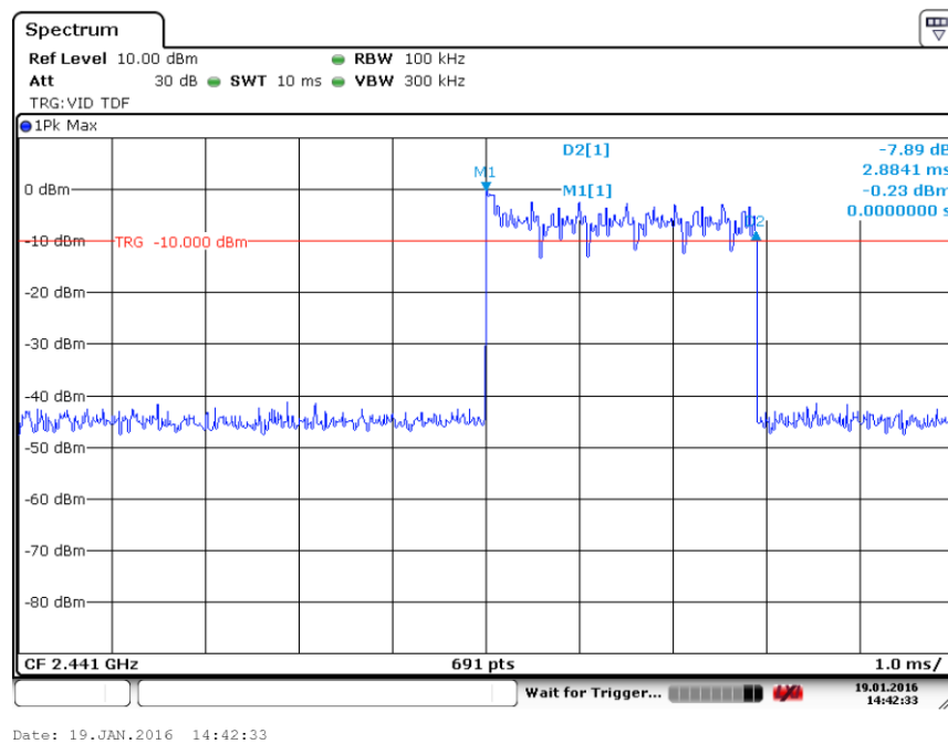
Fig. 83 Time of Occupancy(Dwell Time) ( \pi/4 DQPSK, Ch39)
