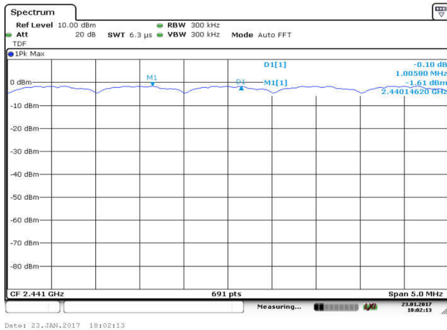
Fig. 111 Carrier Frequency Separation (8DPSK, Ch39)
