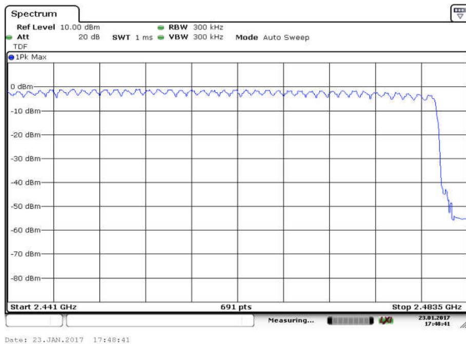
Fig. 106 Hopping channel ch39~78 ( \pi/4 DQPSK, Ch39)
