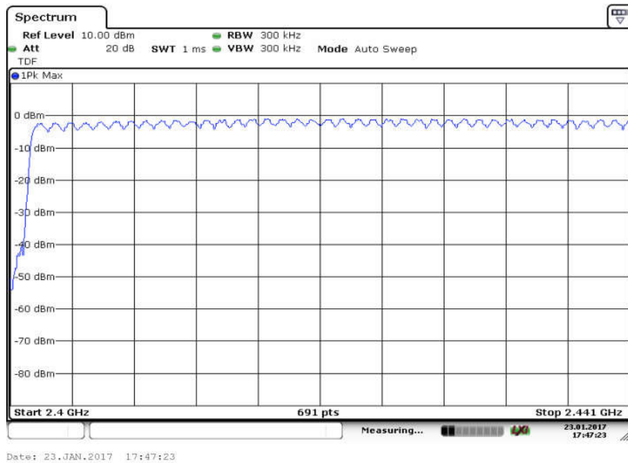
Fig. 105 Hopping channel ch0~39 ( \pi/4 DQPSK, Ch39)
