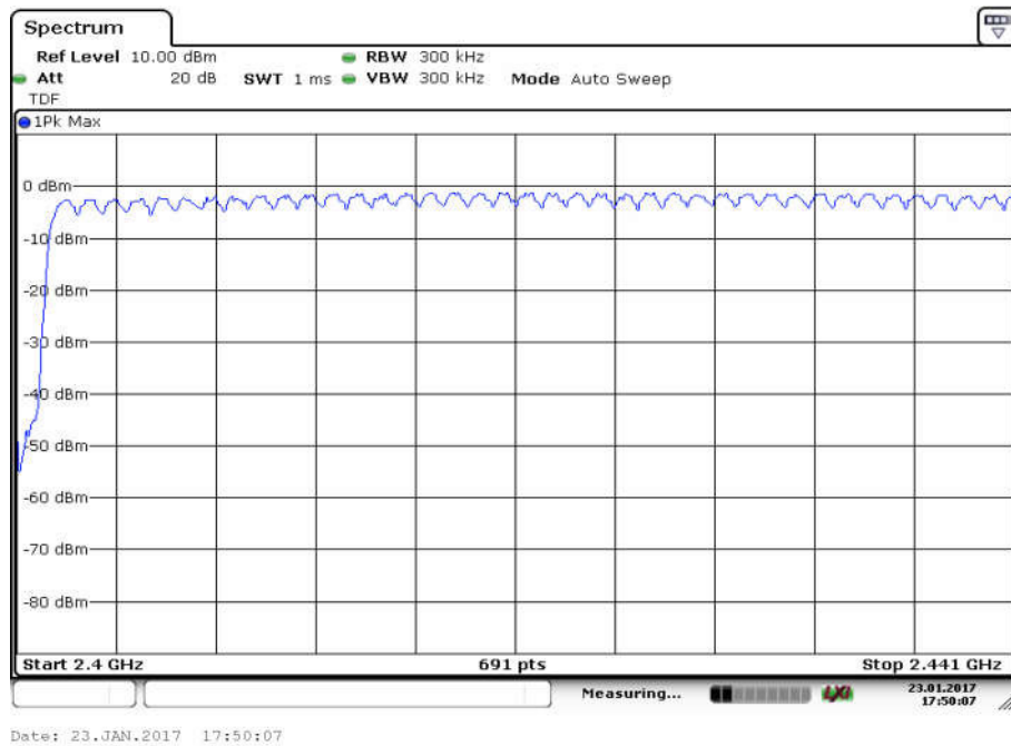
Fig. 107 Hopping channel ch0~39 (8DPSK, Ch39)
