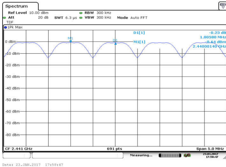
Fig. 109 Carrier Frequency Separation (GFSK, Ch39)
