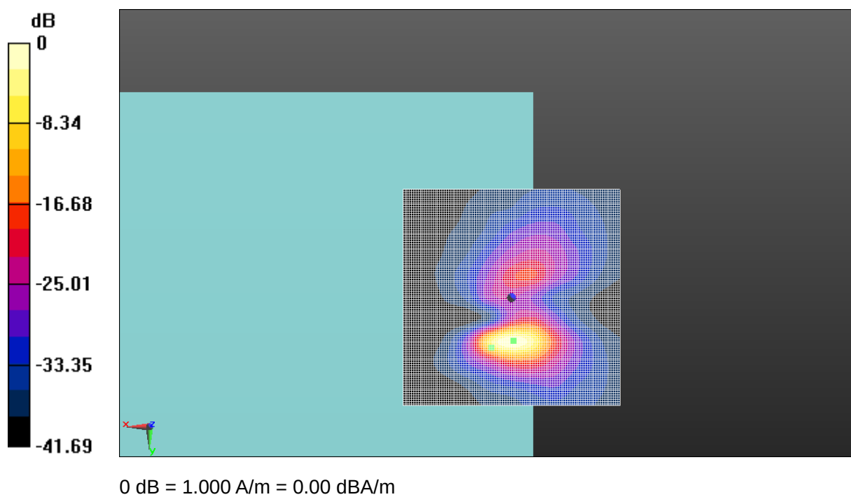
Fig A.34 T-Coil WIFI 5.8G
