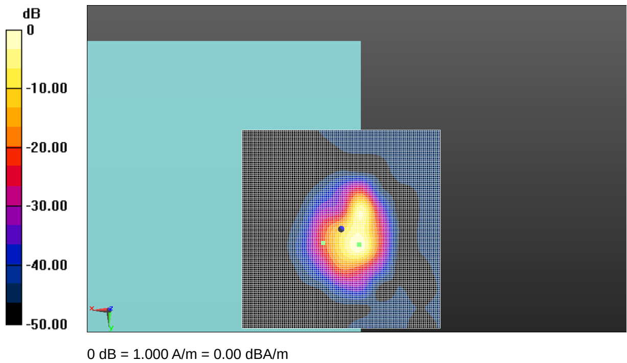
Fig A.49 T-Coil WIFI 5.3G
