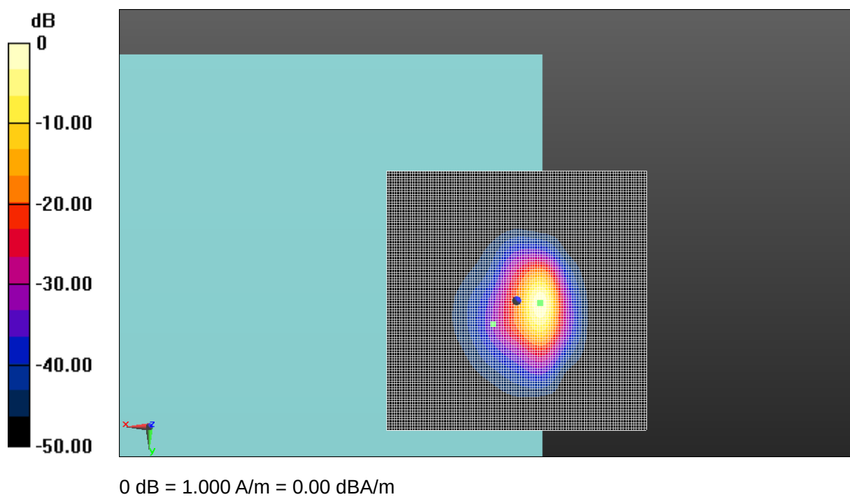
Fig A.31 T-Coil WIFI 5.5G
