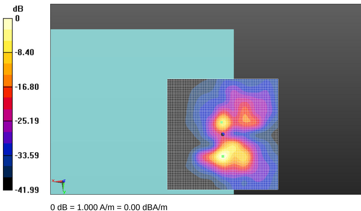
Fig A.50 T-Coil WIFI 5.3G
