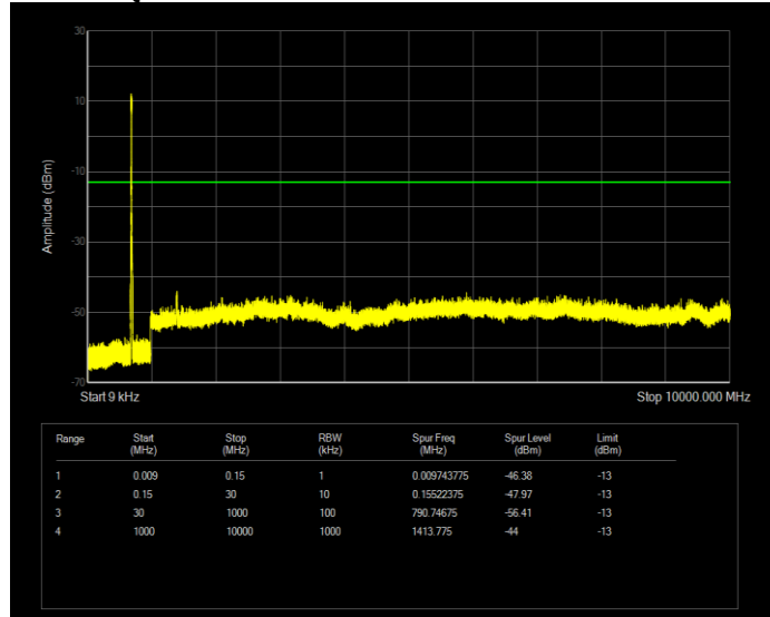
Band12 QAM16 BW=10MHz Channel=23095 RB Size=50 Position=#0
