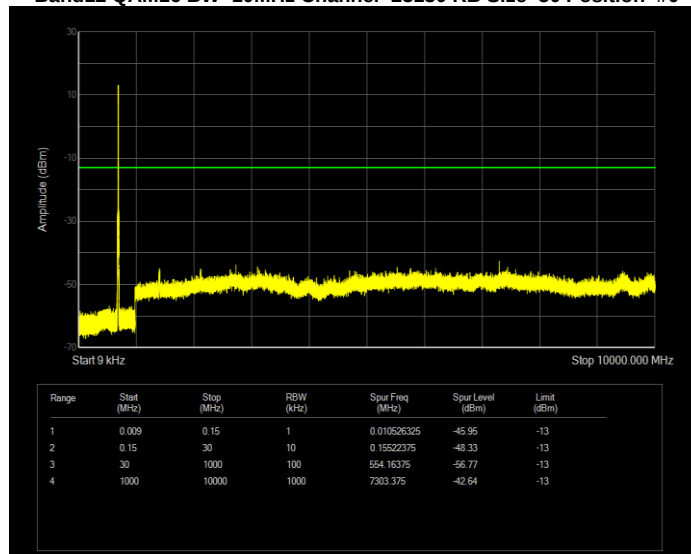
Band12 QAM16 BW=10MHz Channel=23130 RB Size=50 Position=#0
