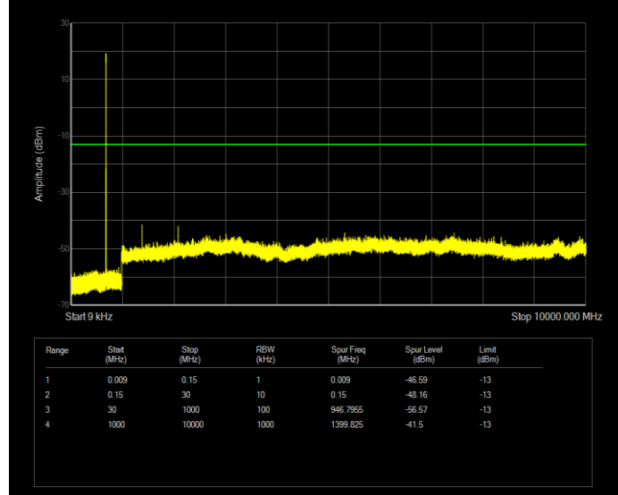
Band12 QAM16 BW=1.4MHz Channel=23095 RB Size=6 Position=#0
