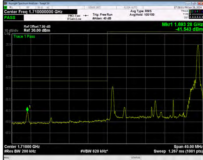
Band4 16QAM BW=20MHz Channel=20050 RB Size=100 Position=#0 Extended
