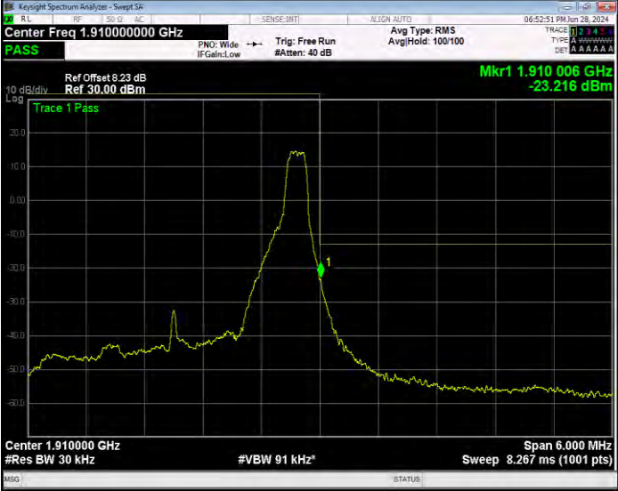
Band2 16QAM BW=3MHz Channel=19185 RB Size=15 Position=#0 Extended
