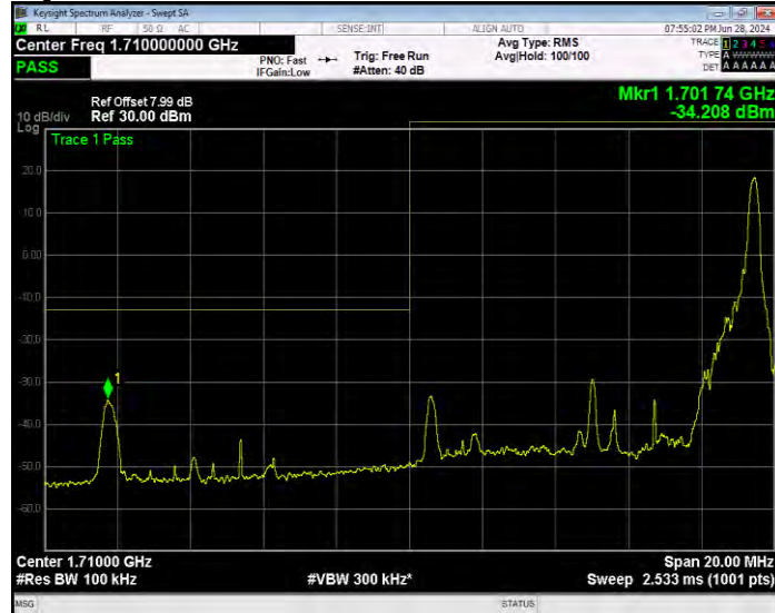
Band4 16QAM BW=10MHz Channel=20000 RB Size=50 Position=#0 Extended
