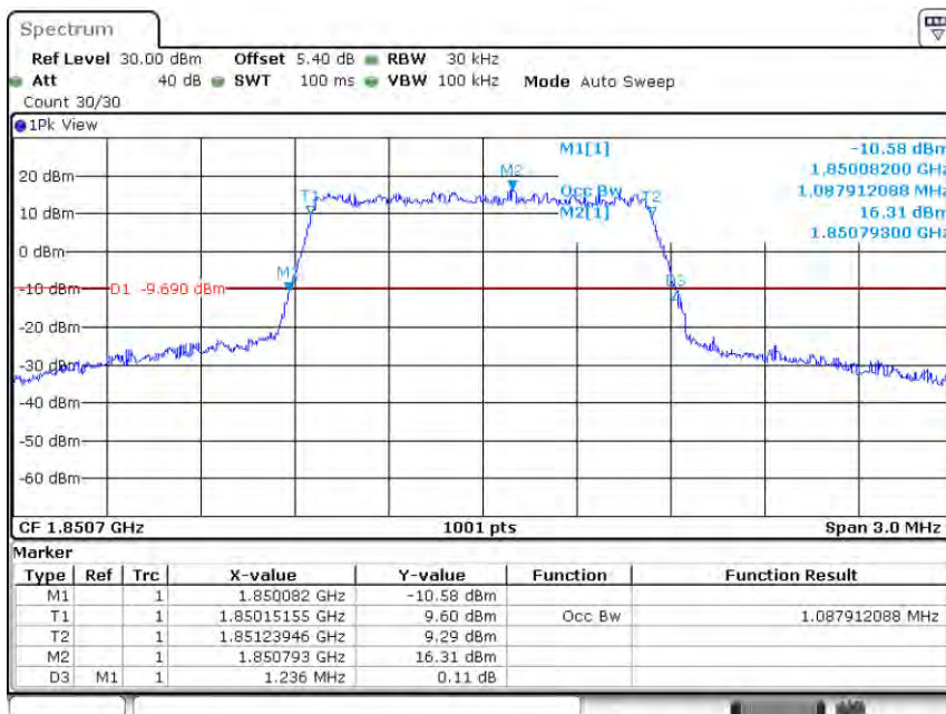
Band25-1.4MHz-QPSK-26047-6RB#0-1.088
