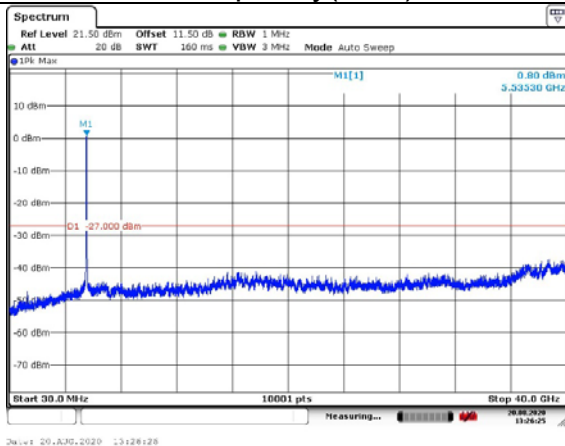
802.11ac VHT80 Carrier frequency(MHz):5530
