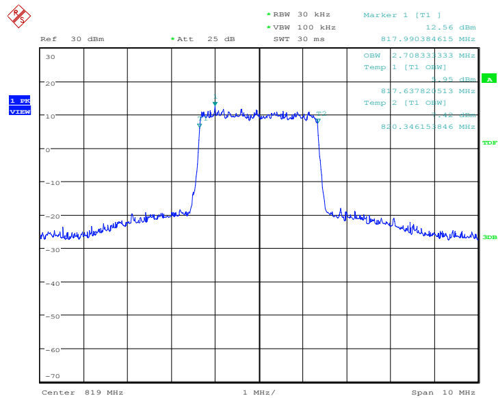
Plot 1.8: LTE Band 26, 3MHz Bandwidth, 16QAM (99% BW)
