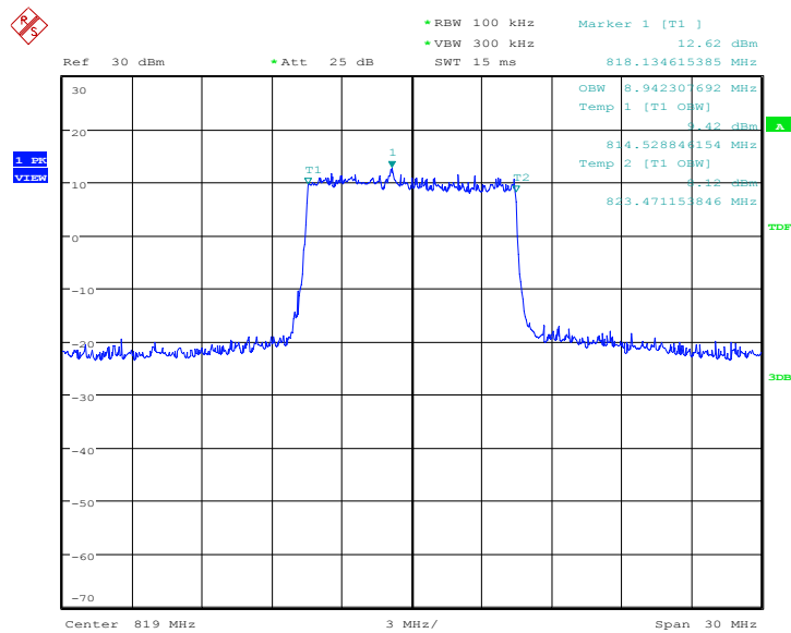
Plot 1.12: LTE Band 26, 10MHz Bandwidth, 16QAM (99% BW)
