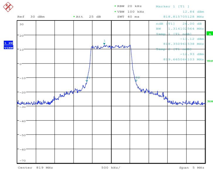
Plot 1.14: LTE Band 26, 1.4MHz Bandwidth, 16QAM (-26dBc BW)
