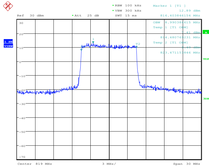
Plot 1.11: LTE Band 26, 10MHz Bandwidth, QPSK (99% BW)
