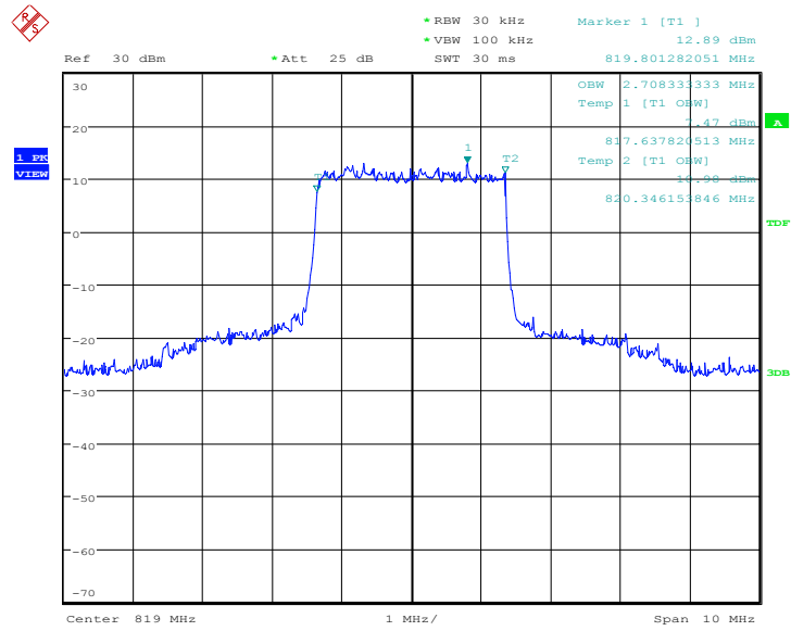
Plot 1.7: LTE Band 26, 3MHz Bandwidth, QPSK (99% BW)
