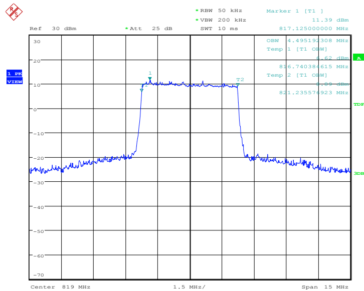
Plot 1.10: LTE band 26, 5MHz Bandwidth, 16QAM (99% BW)
