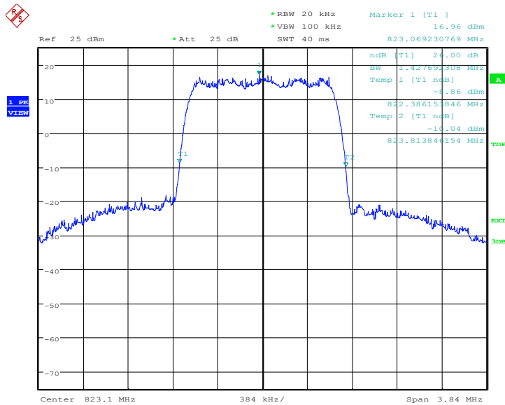
Plot 1.4: Channel 384-Occupied Bandwidth (-26dBc BW)
