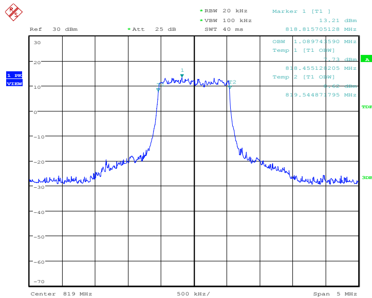
Plot 1.6: LTE Band 26, 1.4MHz Bandwidth, 16QAM (99% BW)
