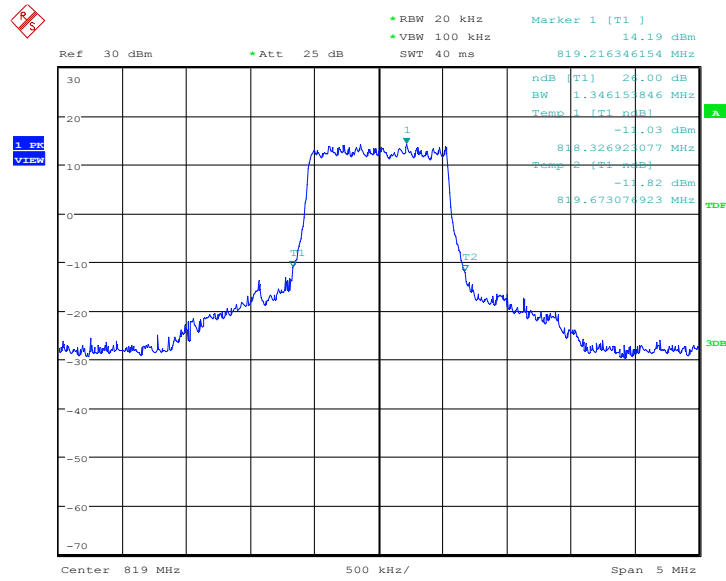
Plot 1.13: LTE Band 26, 1.4MHz Bandwidth, QPSK (-26dBc BW)
