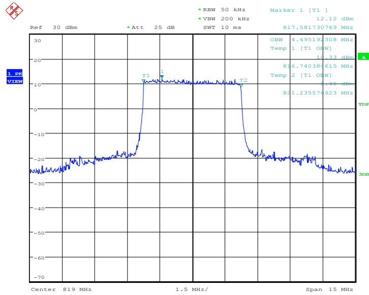
Plot 1.9: LTE band 26, 5MHz Bandwidth, QPSK (99% BW)
