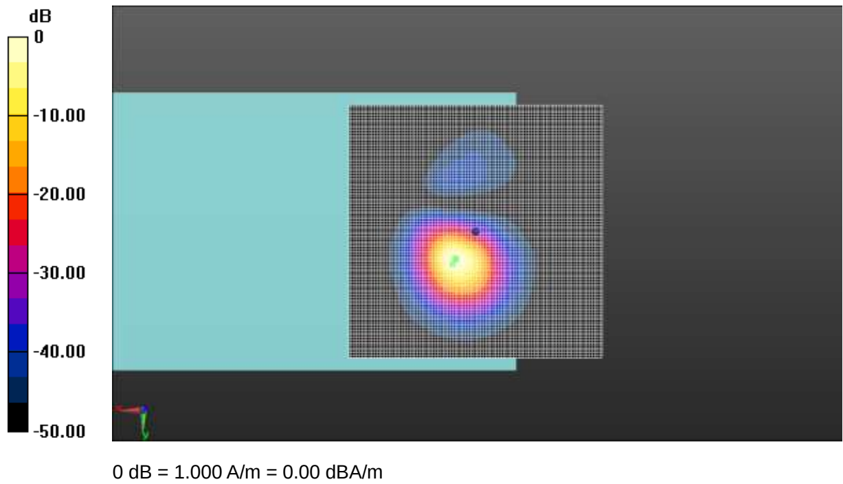
Fig A.30 T-Coil WCDMA Band 2-Z
